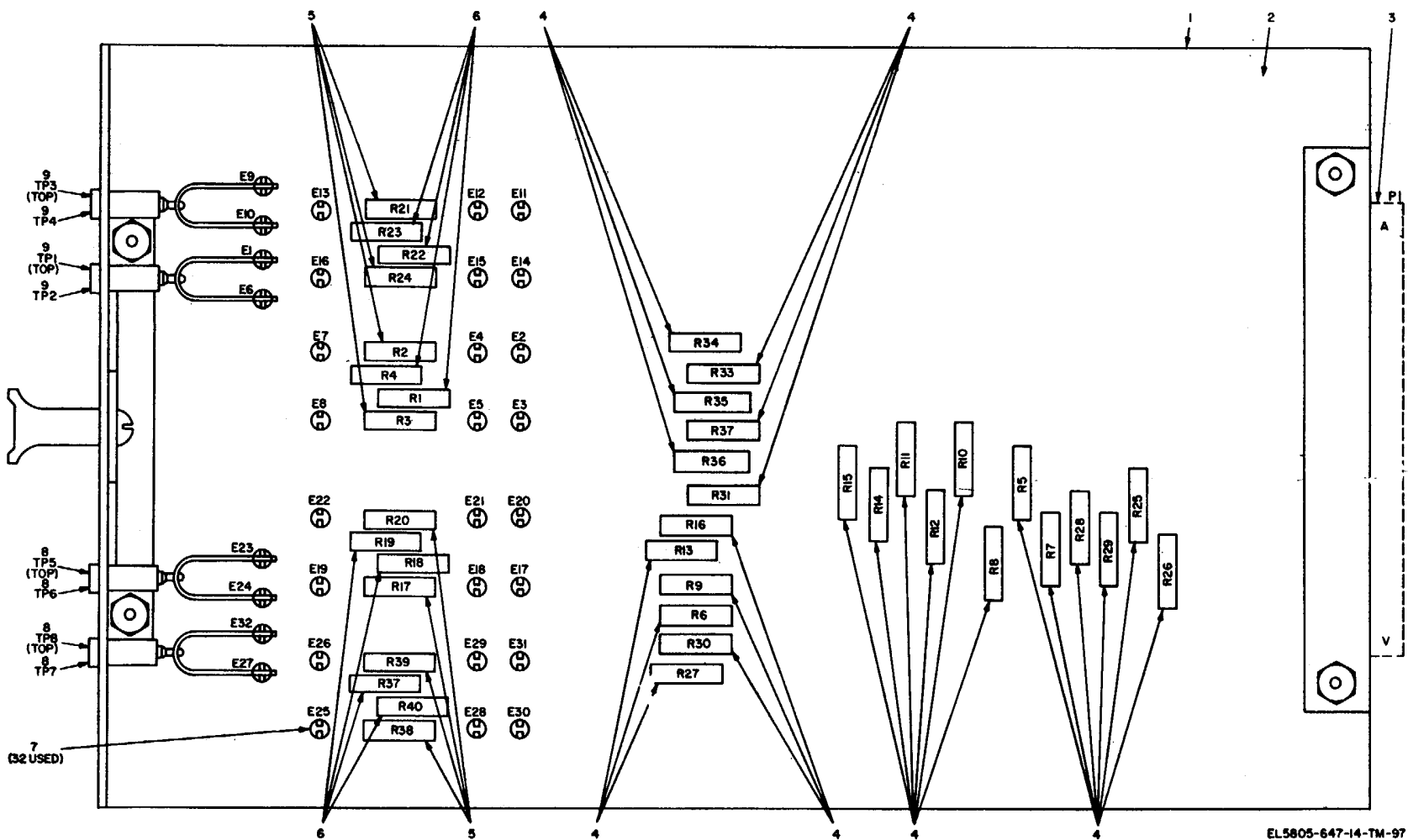
Figure 30. 4-Way/4-wire bridge 40455-03, parts location.
