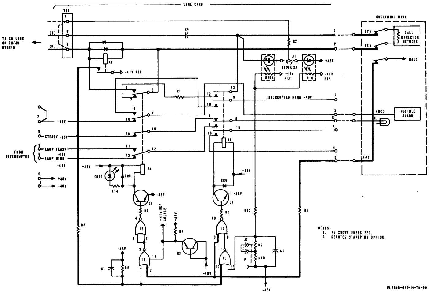
Figure 4-9. Call answered functional diagram.
