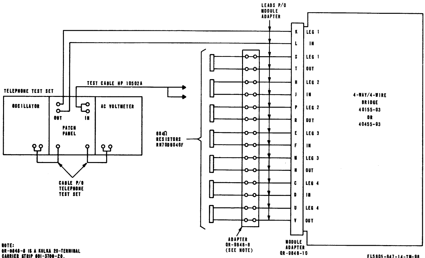
Figure 6-15. 4-Way/4-Wire Bridge 40165-03 and 40455-03, initial test setup diagram.
