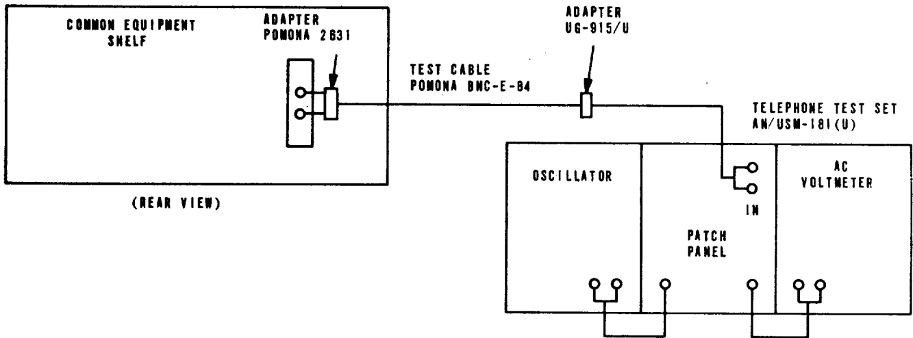
Figure 2-16. SF detector and oscillator, 41063-02, test setup diagram
