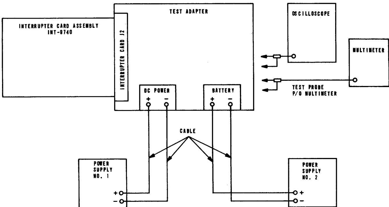
Figure 6-22. Interrupter Card Assembly INT-9740, test setup diagram.
