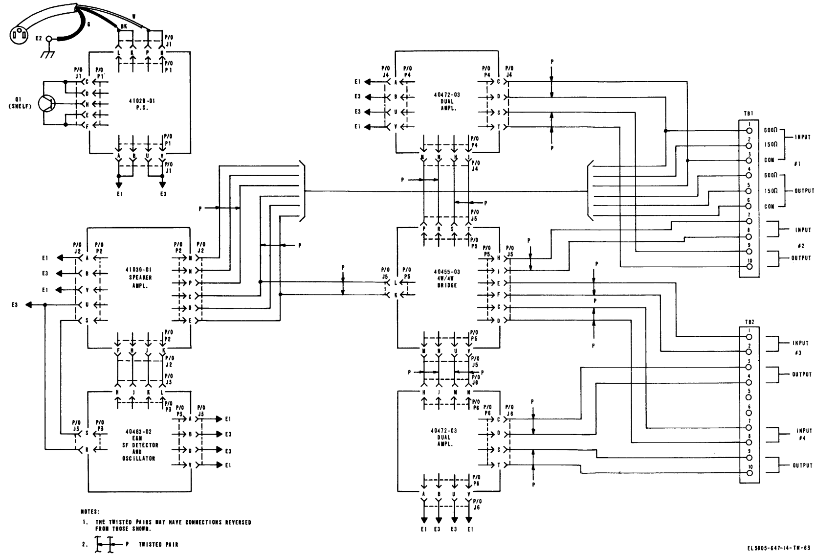
Figure FO-6. Local Orderwire Unit 41010-97, interconnection wiring diagram.
