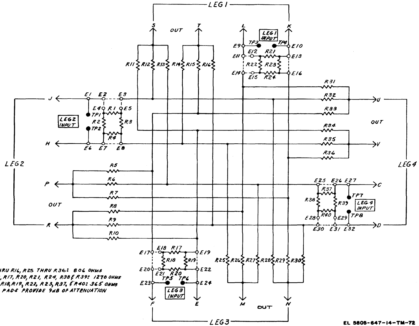
Figure FO-16. 4-way/4-wire bridge 40155/40455-03, schematic diagram.
