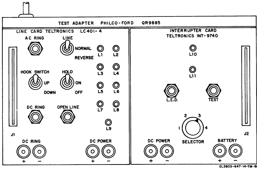
Figure 6-5. Test Adapter QR-986, pictorial diagram.
