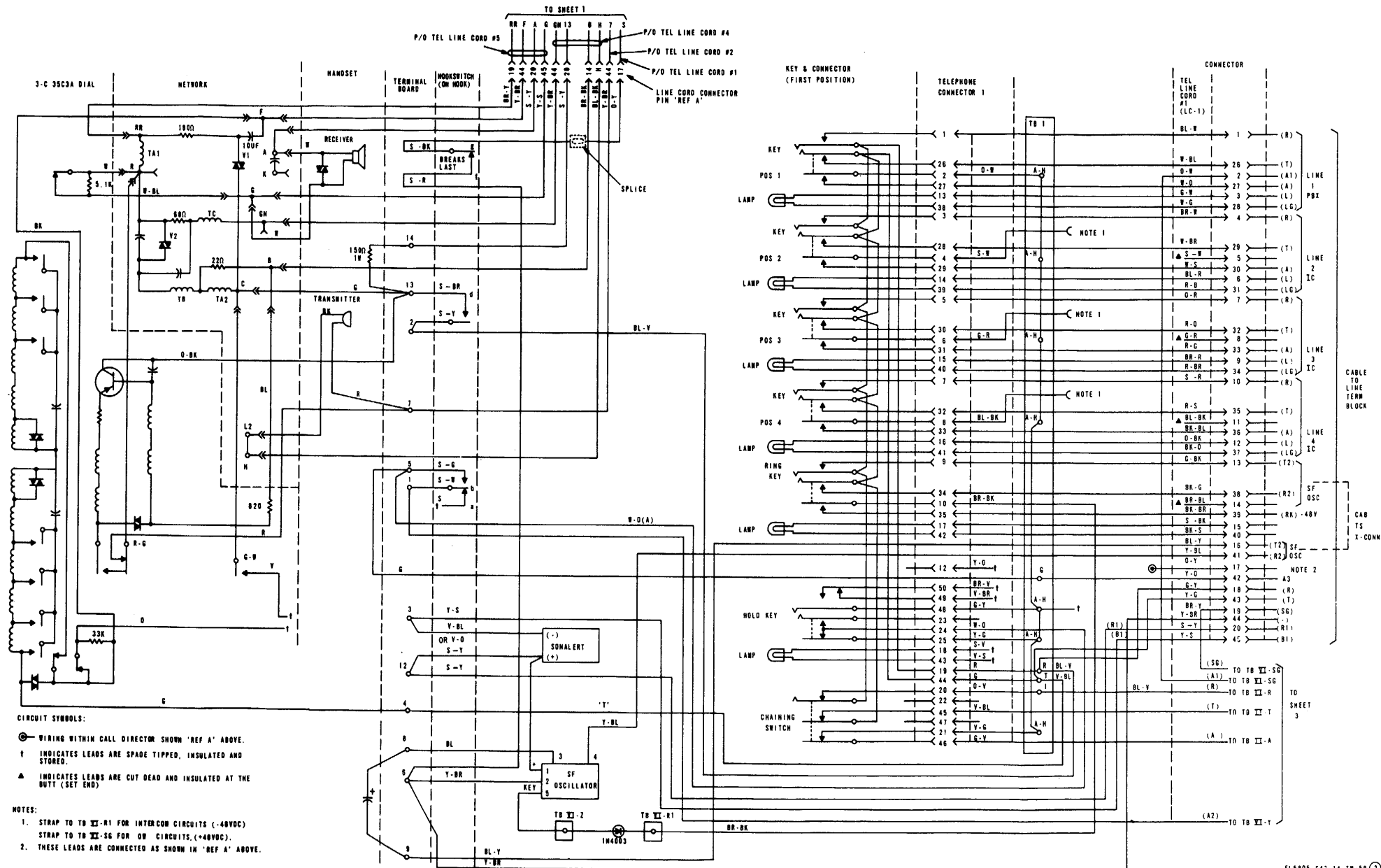
Figure FO-1(2). Express-Link-Local Orderwire Unit TA-928/FSC, wiring diagram (sheet 2 of 4).
