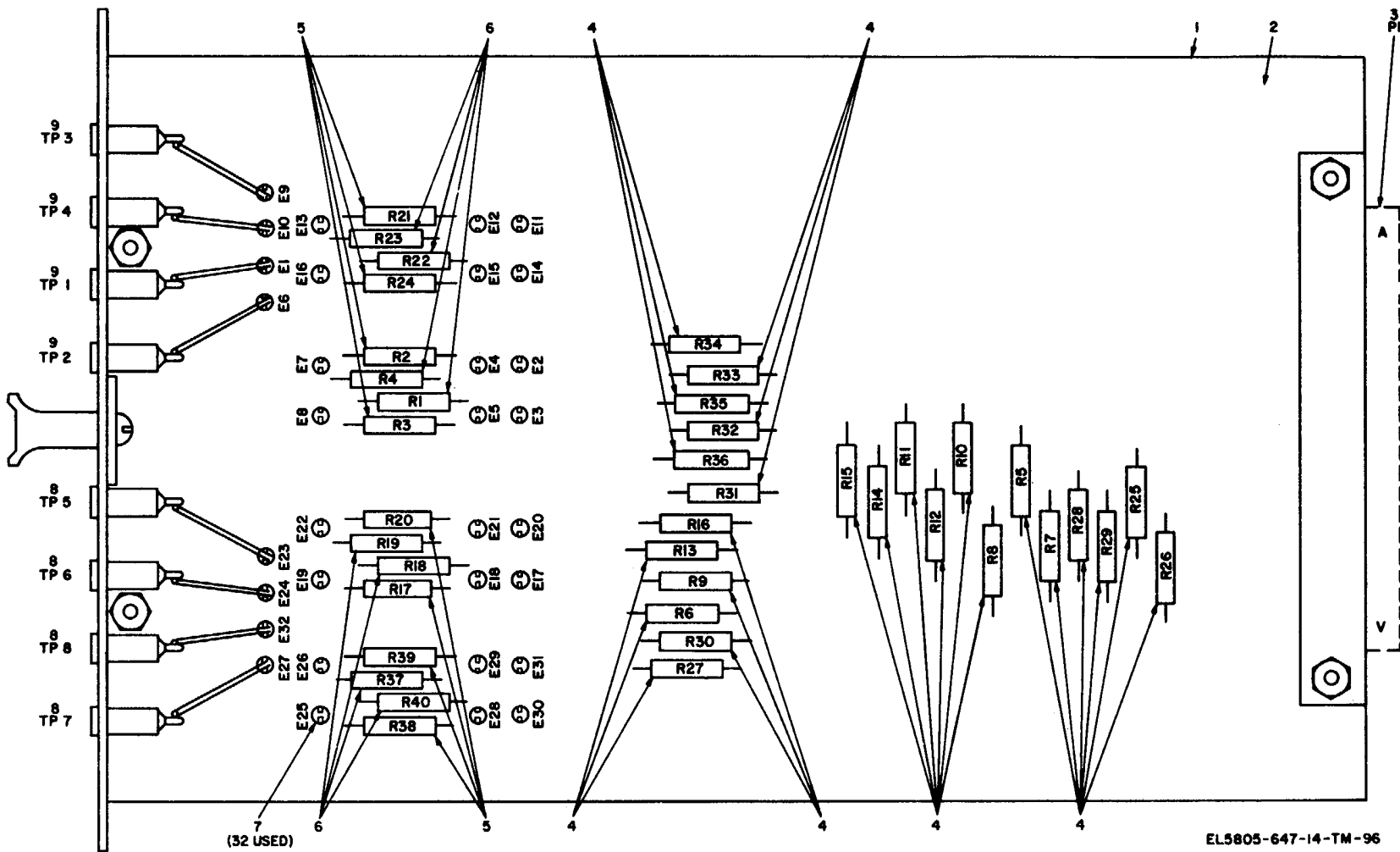
Figure 34. 4-Way/4-wire bridge 40155-03, parts location.
