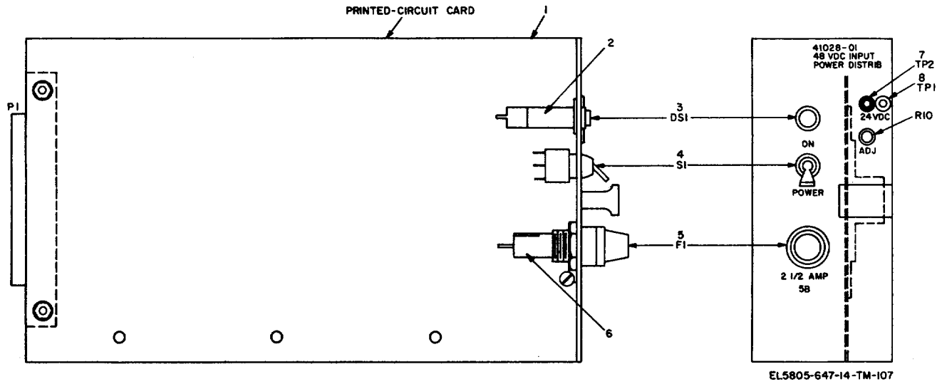
Figure 28. Power supply 41028-01, parts location.
