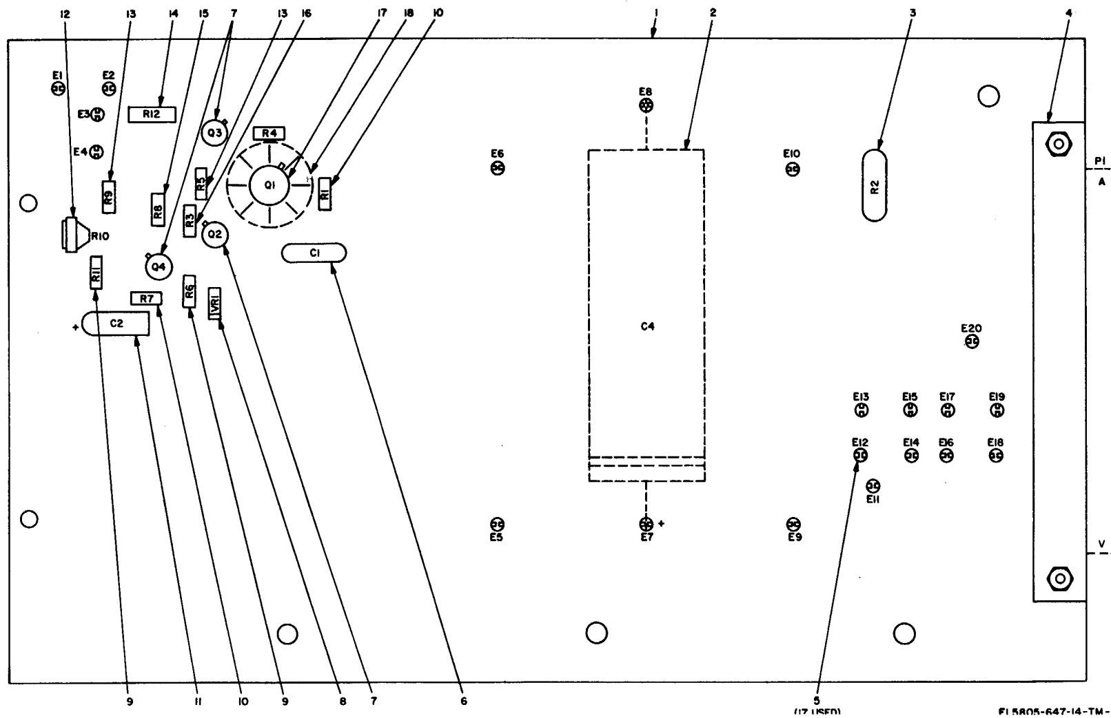
Figure 38. Printed circuit card for power supply 41029-01, parts location.
