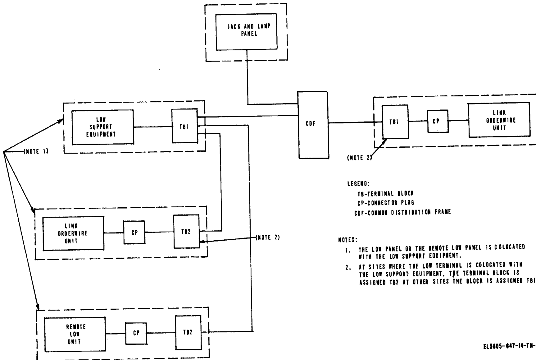
Figure 2-2. LOW site installation procedures pictorial identification.
