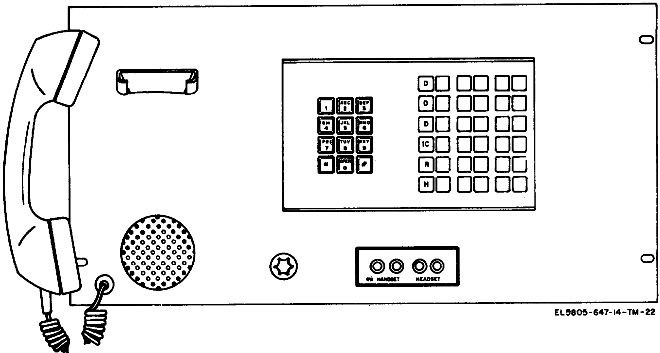
Figure 3-4. Remote Link Orderwire Unit TA-924/FSC (front view).
