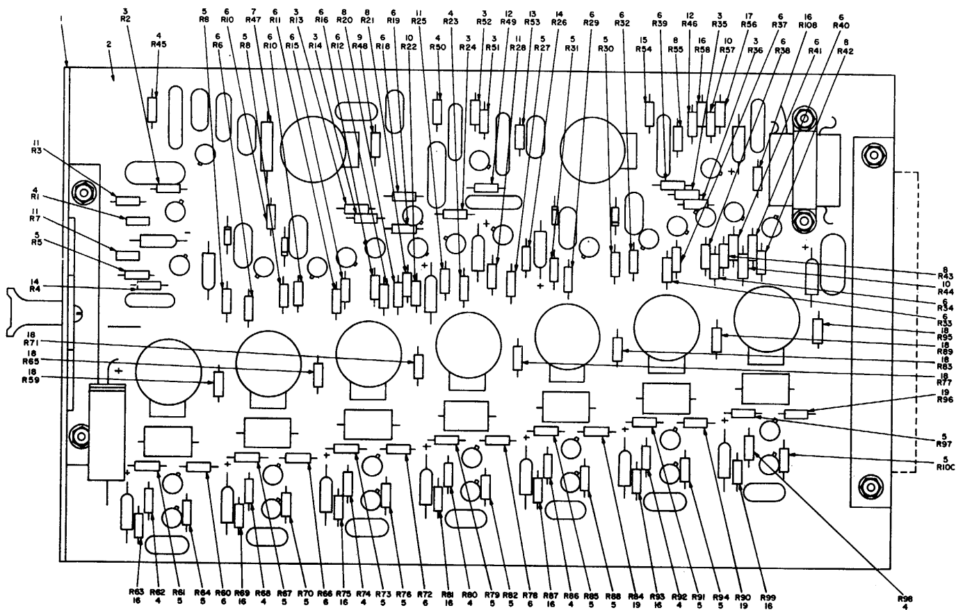
Figure 19. Tone receiver 40452-01, resistor location.
