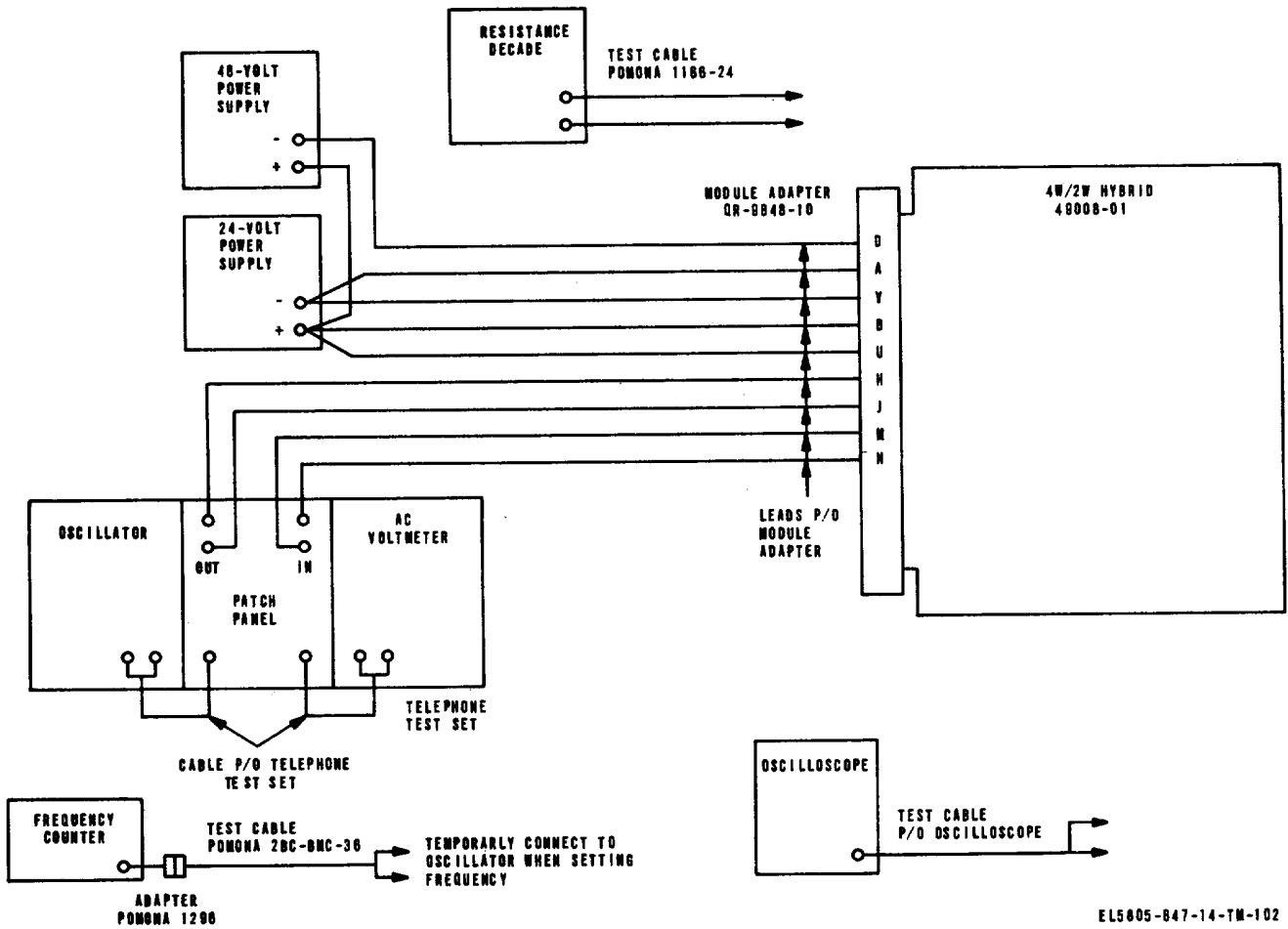
Figure 6-17. 4-Wire/2-Wire Hybrid 49U'082-, initial test setup lagrm.
