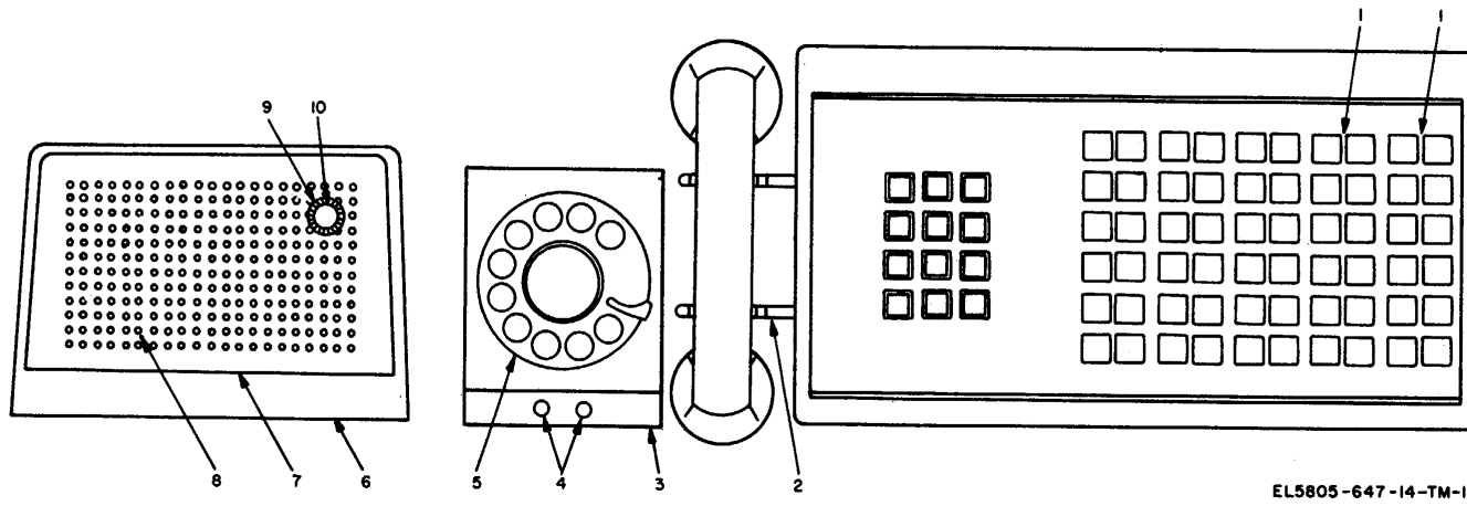
Figure 12. Call director, dial assembly and speaker assembly, parts location.
