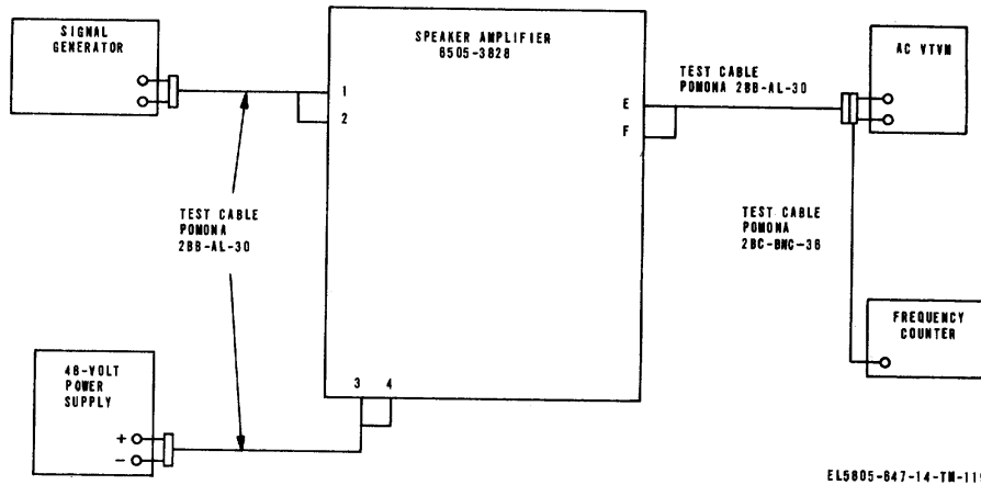
Figure 6-26. Speaker Amplifier Unit 65065-3828, initial test setup diagram.
