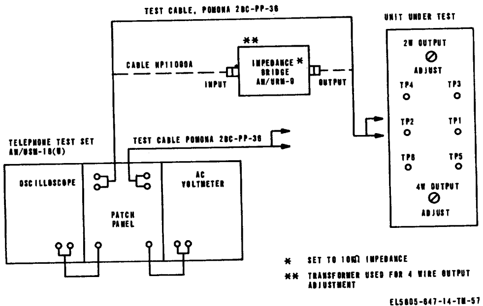
Figure 2-15. 2W/4W hybrid, 49008-02, test setup diagram.
