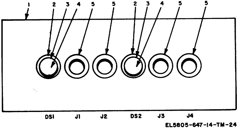
Figure 42. Jack and lamp JLP-1 (front view ), parts location
