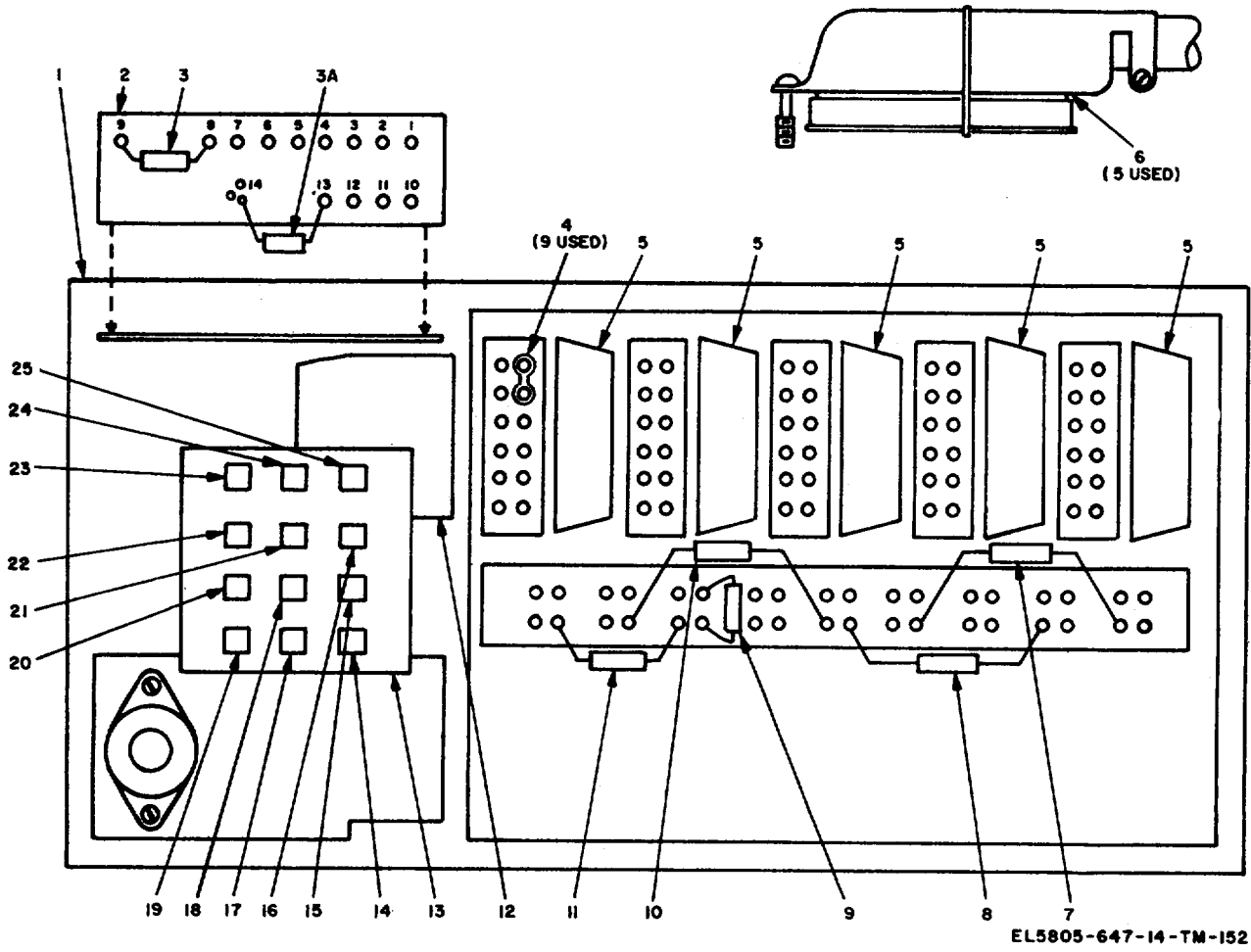
Figure 2. Cal director assembly, parts location.
