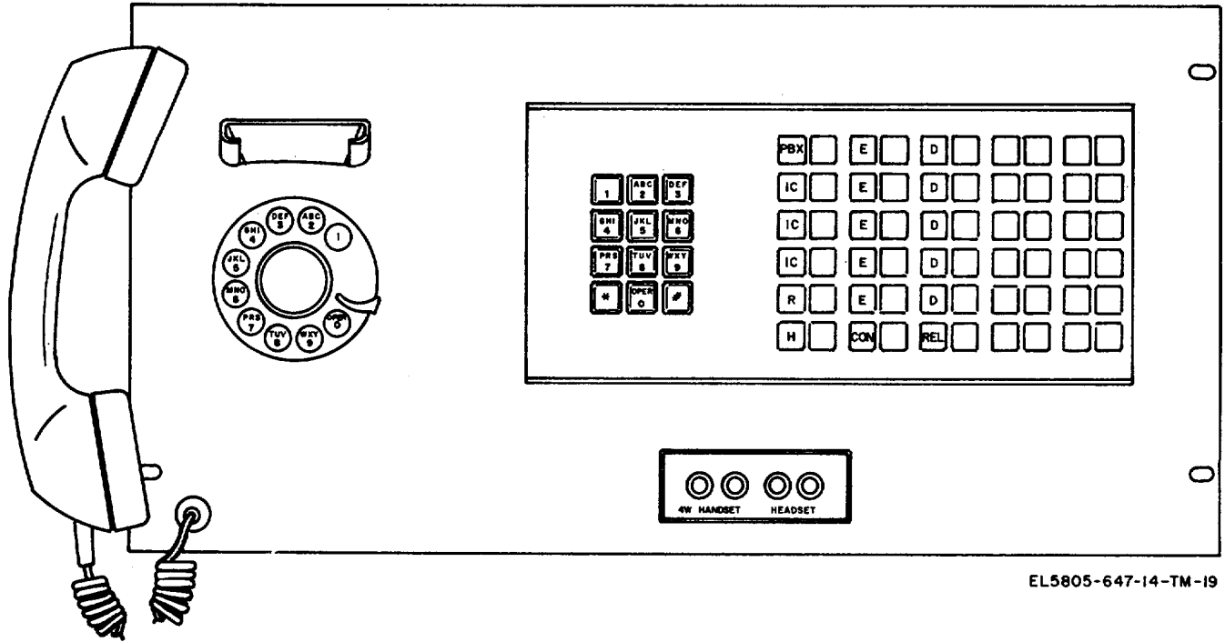
Figure 1-2. Express-Link-Local Order Wire Unit TA-923/FSC.
