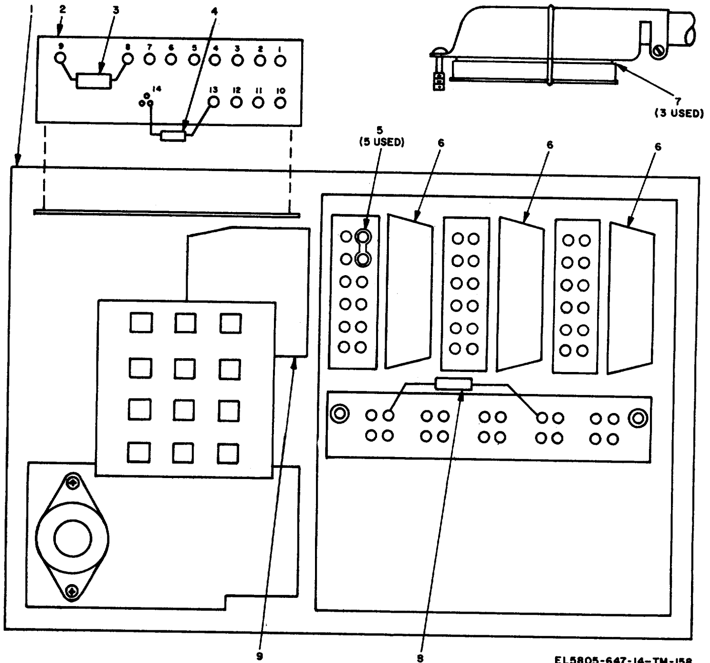
Figure 9. Call director assembly, parts location.
