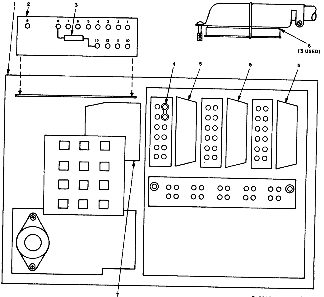
Figure 7. Call director assembly, parts location.
