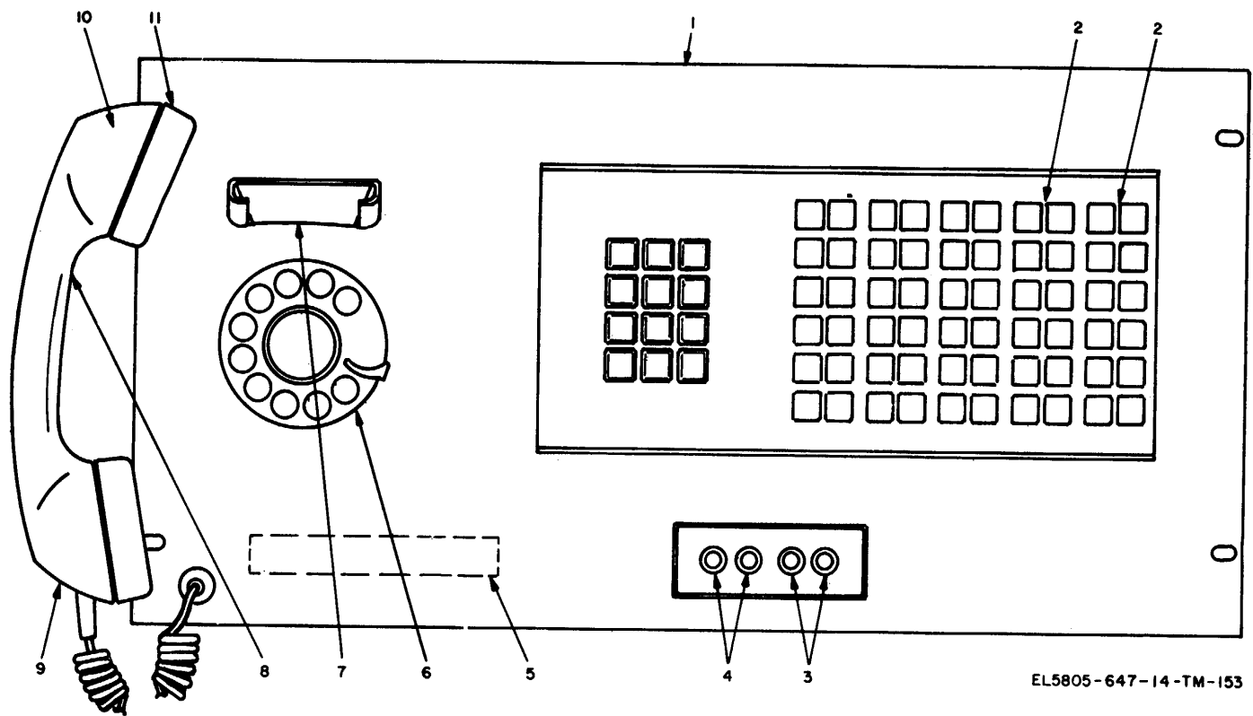
Figure 4. Call director panel assembly and handset, parts location.
