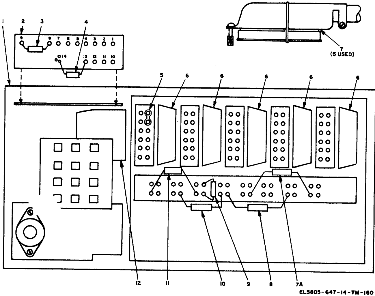
Figure 11. Call director assembly, parts location.
