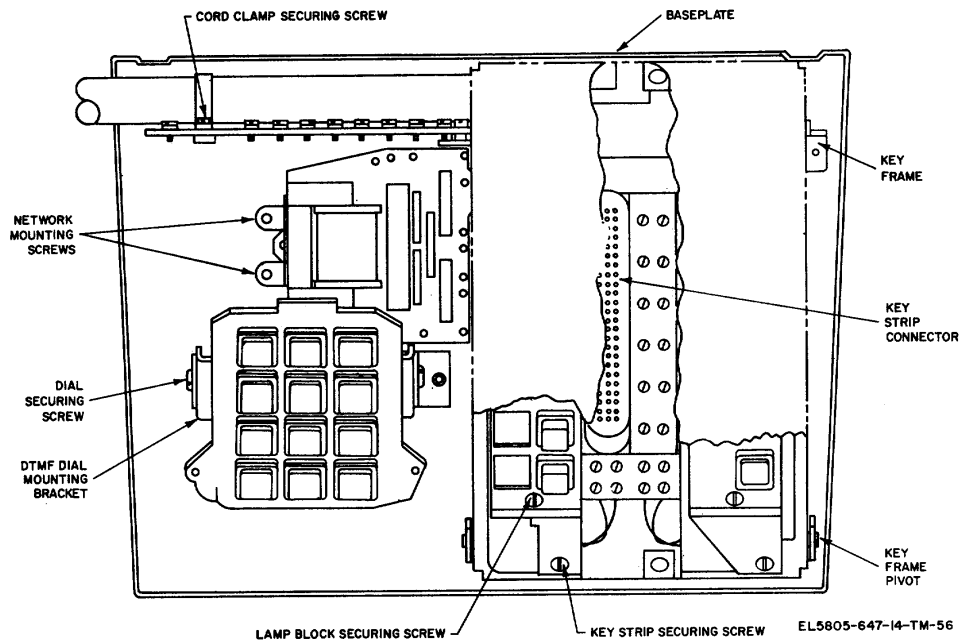
Figure 5-8. 18 button key frame, component mounting
