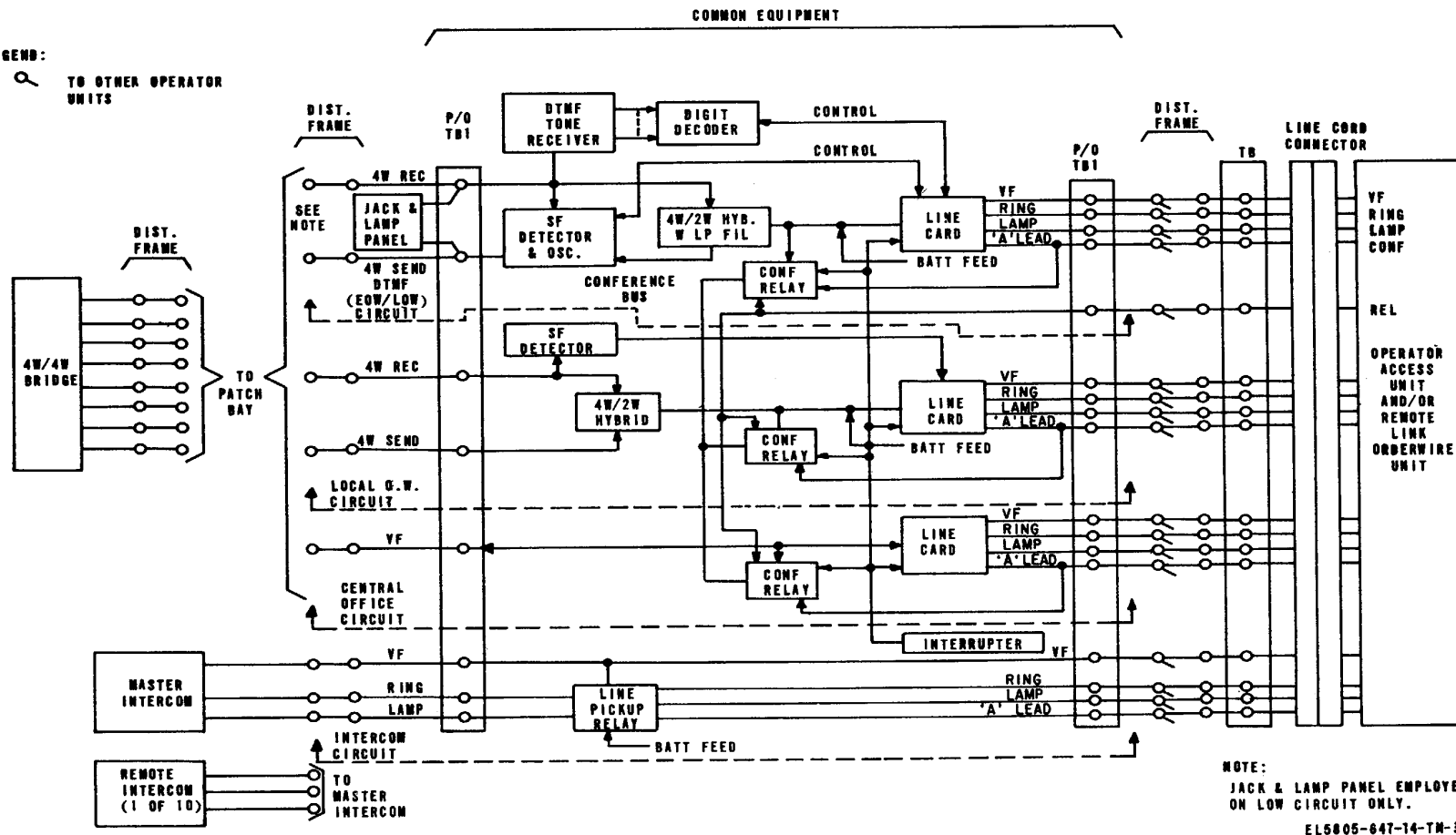
Figure 4-1. Oderwire-Intercommunication Termination Unit TA-918(V)/FSC (EOW site), block diagram
