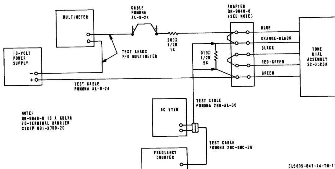
Figure 6-23. Tone Dial Assembly SC-35C3A, performance test setup diagram.
