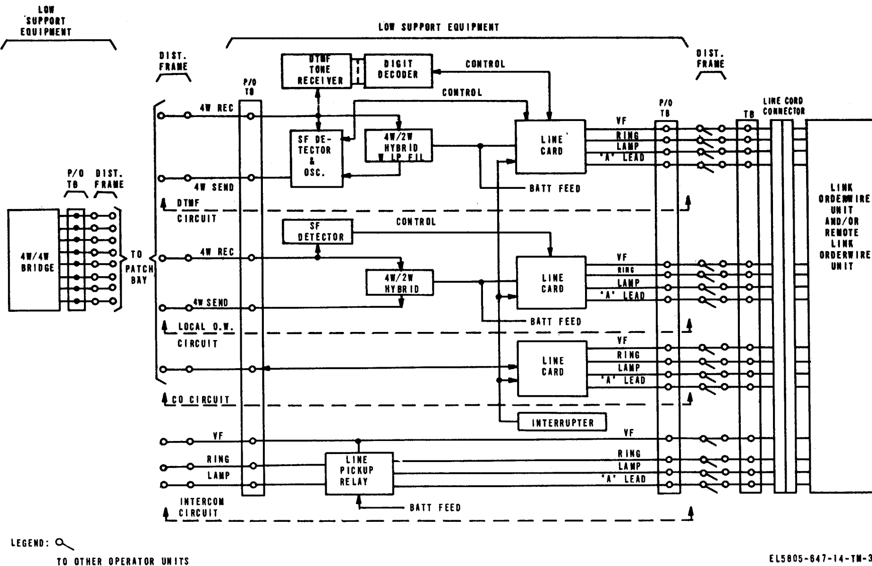
Figure 4-3. Orderwire Intercommunication Termination Unit TA-930(V)/FSC (LOW site), block diagram.
