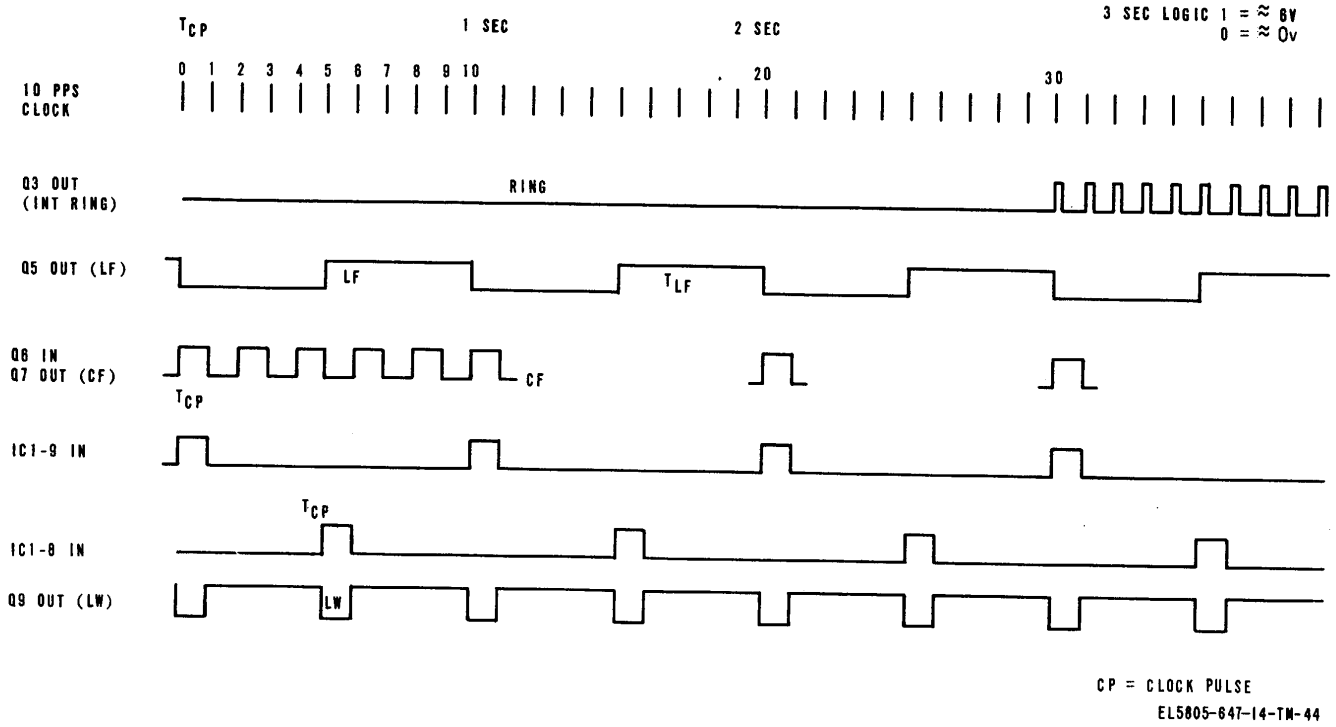
Figure 4-12. Interrupter INT-9740, timing diagram.
