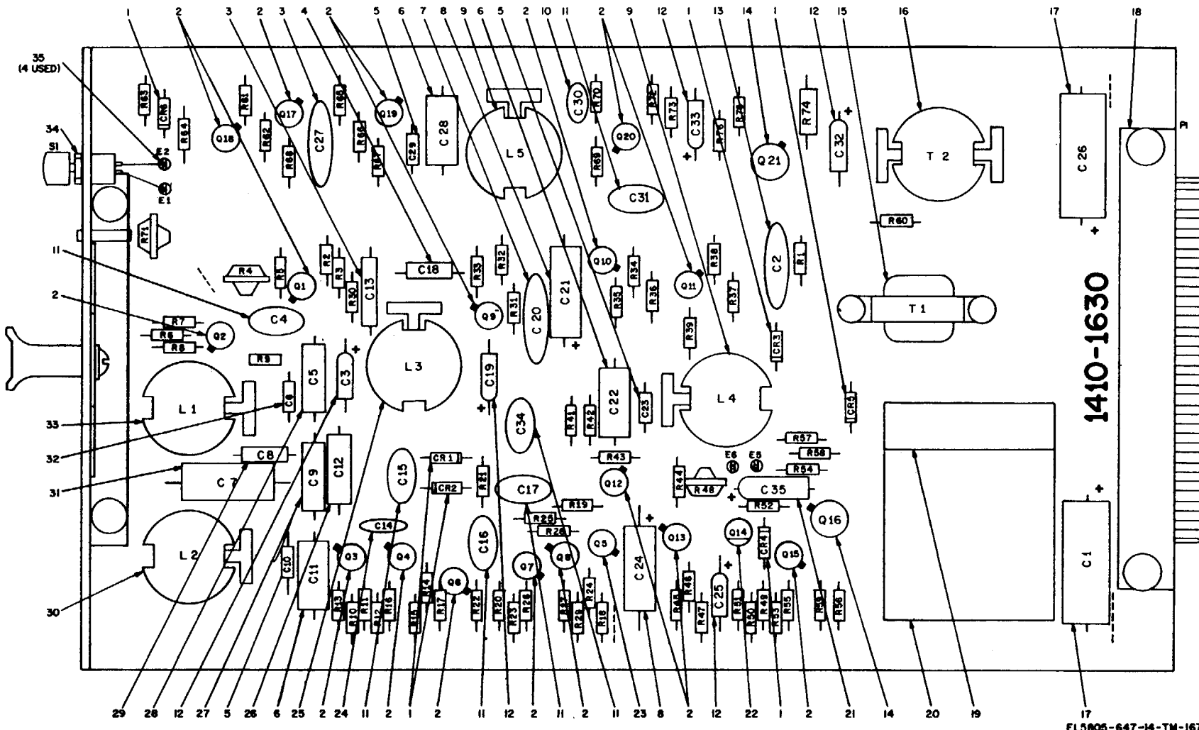
Figure 23. SF detector and oscillator 41063-02, parts location.
