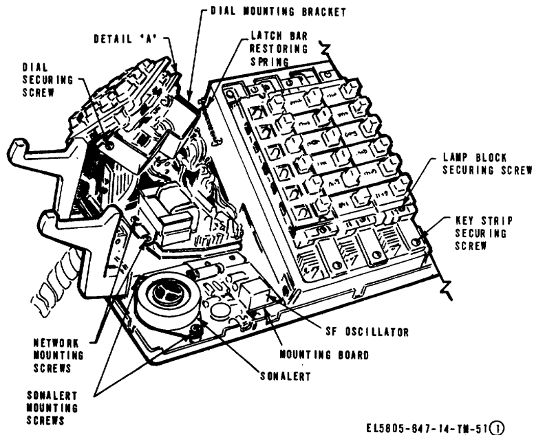
Figure 5-7 (1). 30 button key frame, component mounting (sheet 1 of 2).
