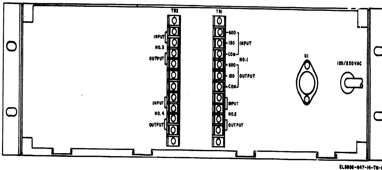
Figure 2-9. Local Orderwire Unit 41010-97, connection terminals (rear).
