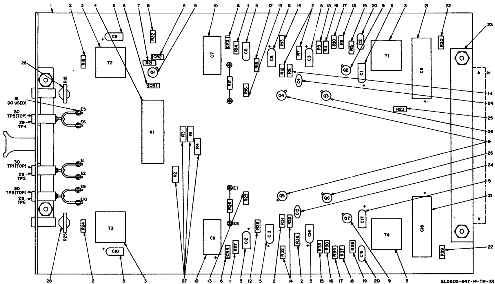
Figure 24. 4-Wire/2-wire hybrid 49008-01, parts location.
