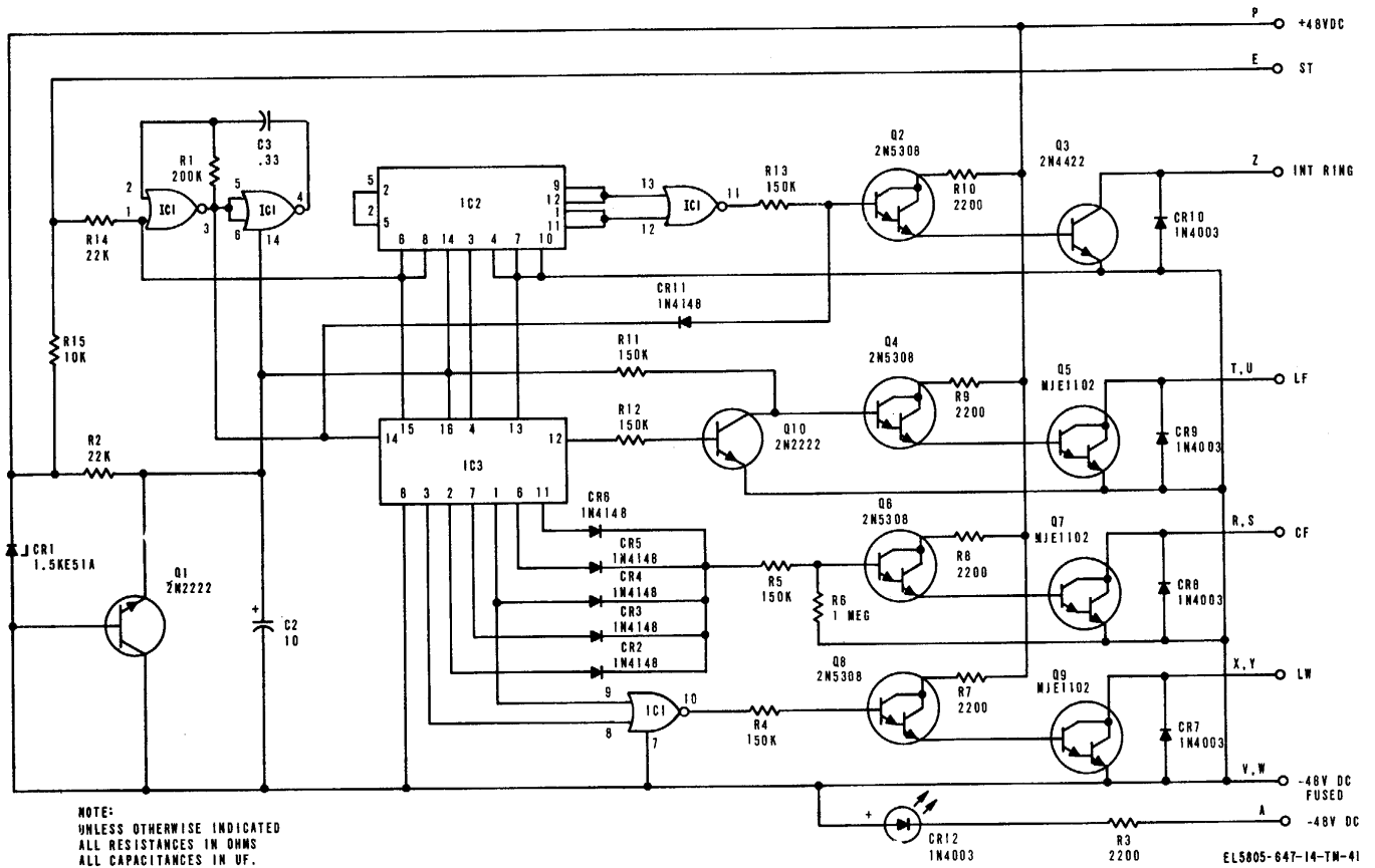
Figure 4-11. Interrupter INT-9740, schematic diagram.
