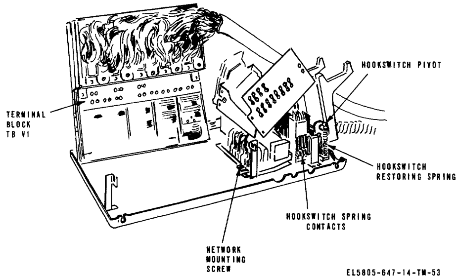
Figure 5-6. Express-Link-Local-Order Wire Unit TA-923/FSC, key frame and hookswitch details and parts location.
