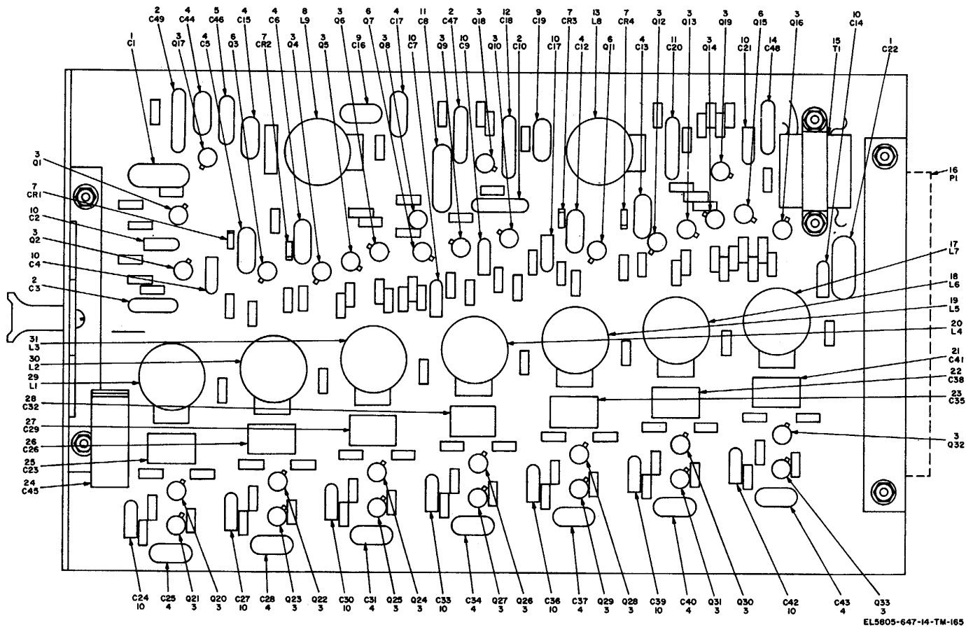
Figure 20. Tone receiver 40452-01, parts location.
