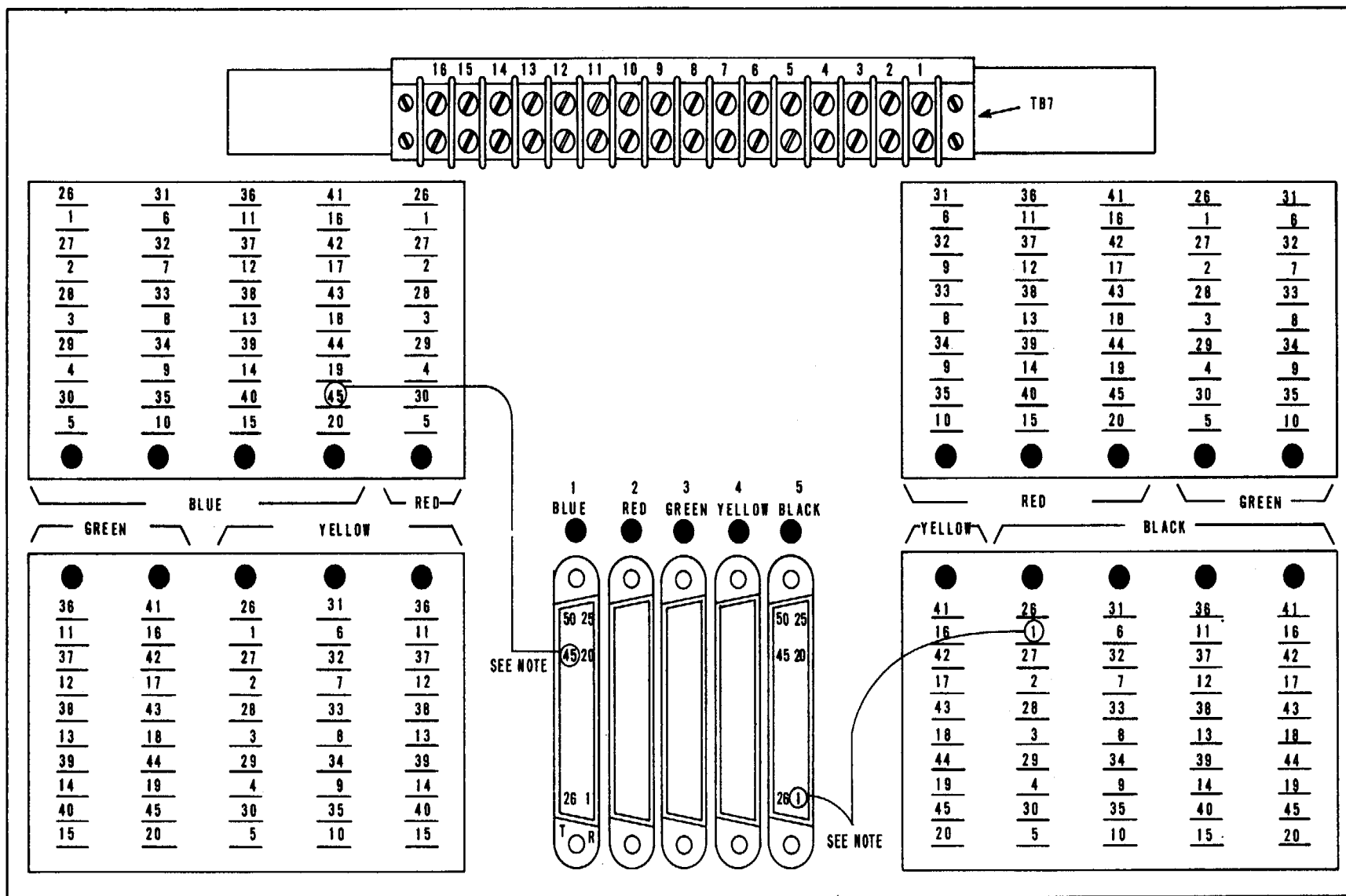
Figure 2-5. Express-Link-Local Order Wire Unit TA-928/FSC, connector block.
