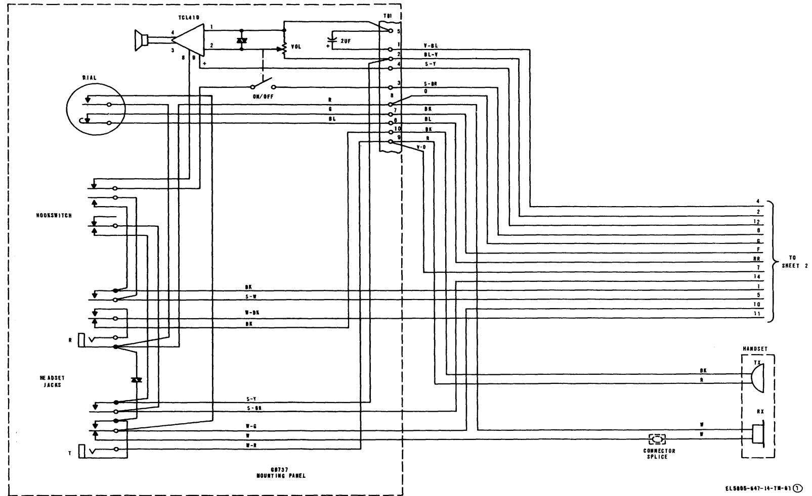
Figure FO-4(1). Link Orderwire Unit TA-925/FSC, wiring diagram (sheet 1 of 3).
