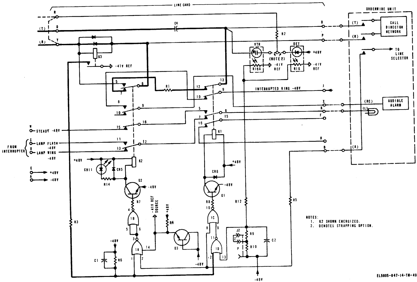
Figure 4-10. Call on hold functional diagram.
