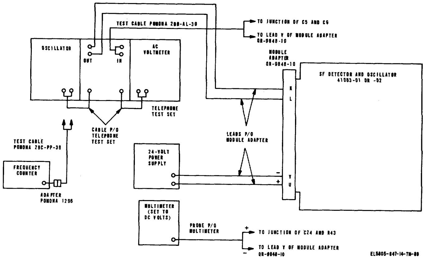
Figure 6-10. S. F. detector initial test setup diagram.
