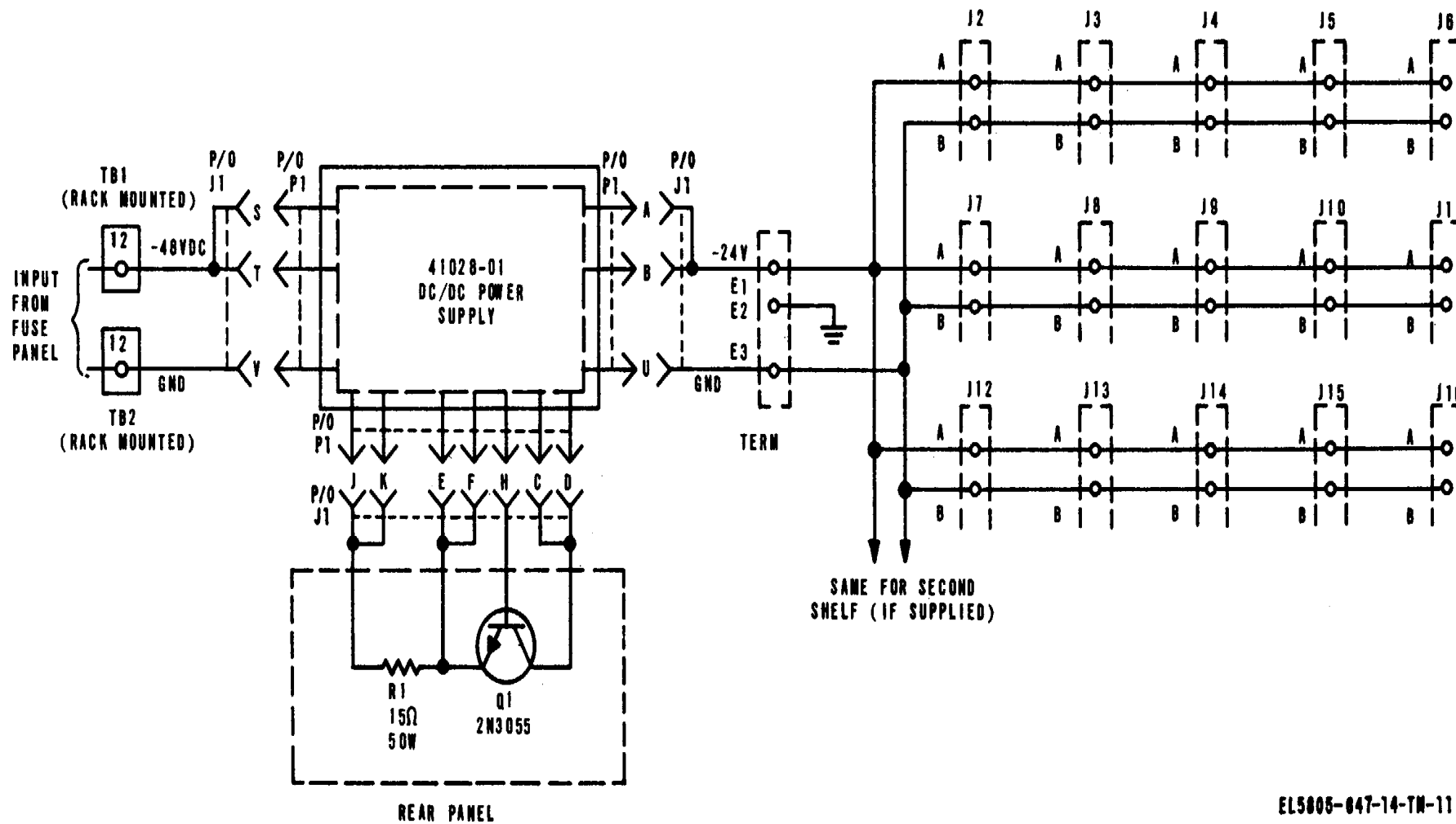
Figure 2-3. Common equipment shelves, dc/dc power supply distribution.
