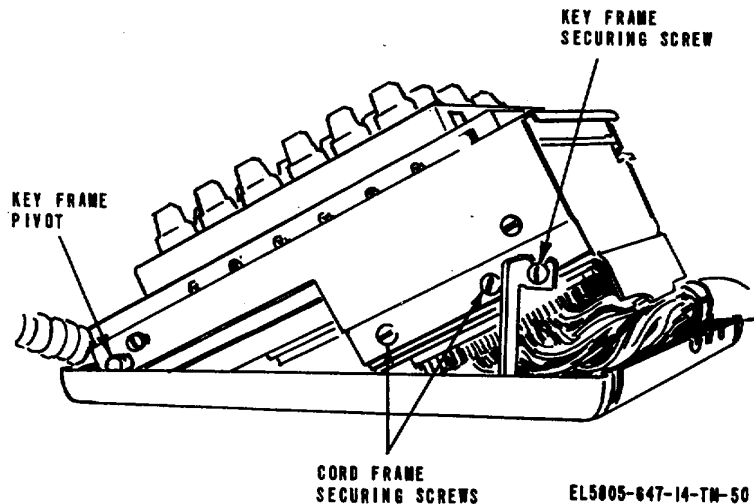
Figure 5-5. Typical frame securing screws, parts location.
