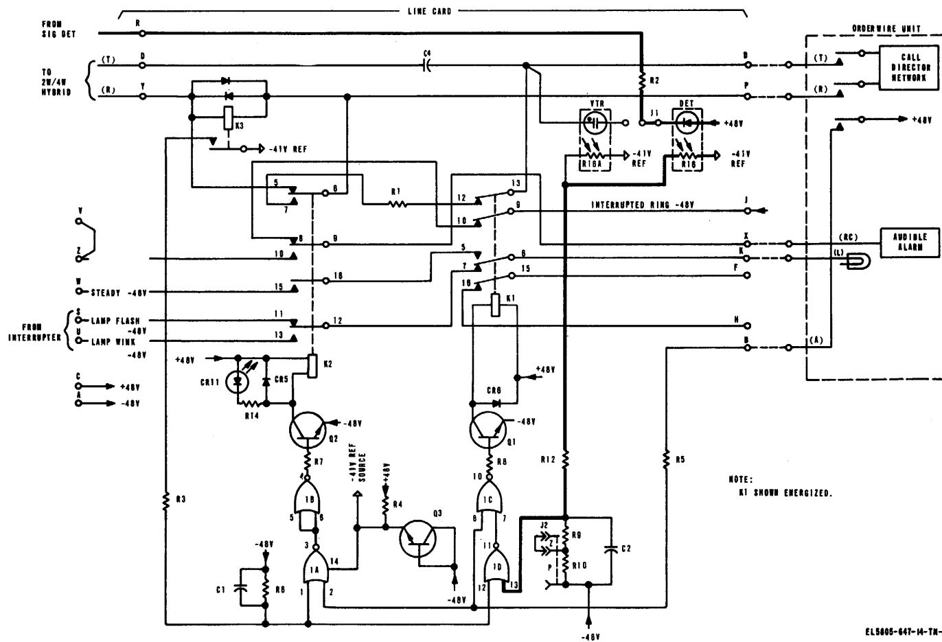
Figure 4-8. DTMF and E & M incoming ring, functional diagram.
