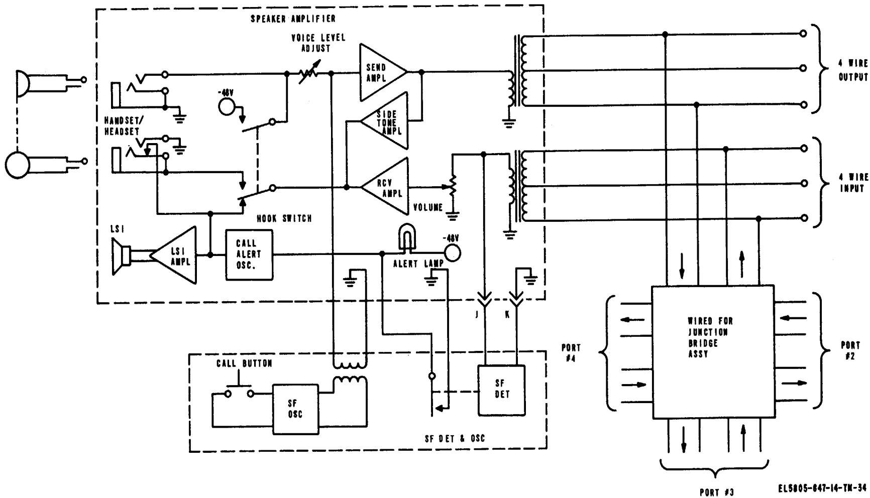
Figure 4-4. Local Orderwire Unit 41010-97, functional block diagram. 4-9
