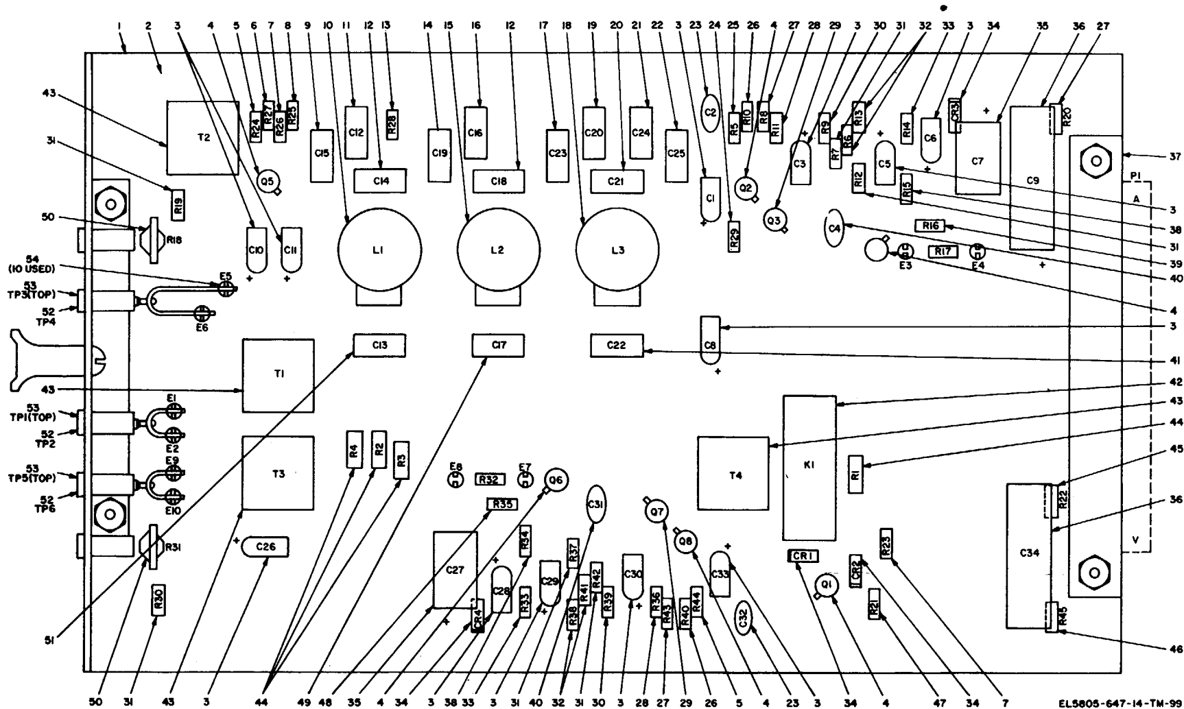
Figure 25. 4-Wire/2-wire hybrid with low-pass filter 49008-02, parts location
