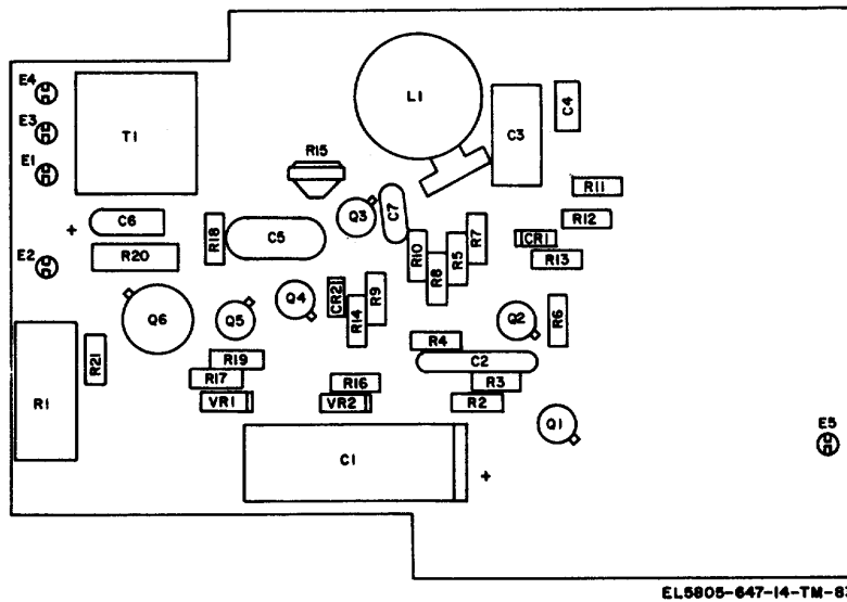
Figure 6-7. S. F. Oscillator 49009-01, parts location diagram.
