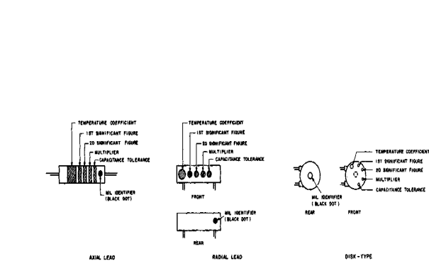
C. COLOR CODE MARKING FOR MILITARY STANDARD CAPACITORS.
