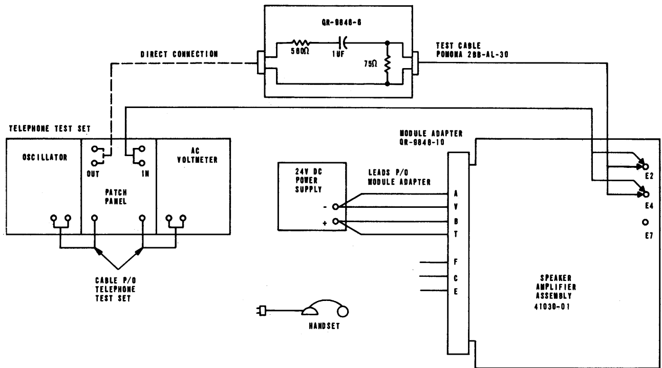
Figure 6-9. Speaker Amplifier Assembly 4103001, test setup diagram.
