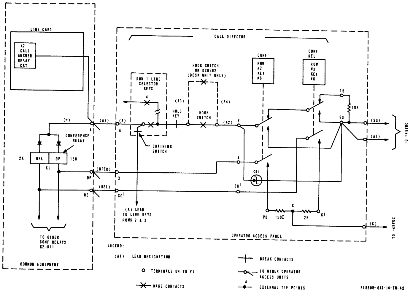
Figure 4-13. Conference functional diagram.
