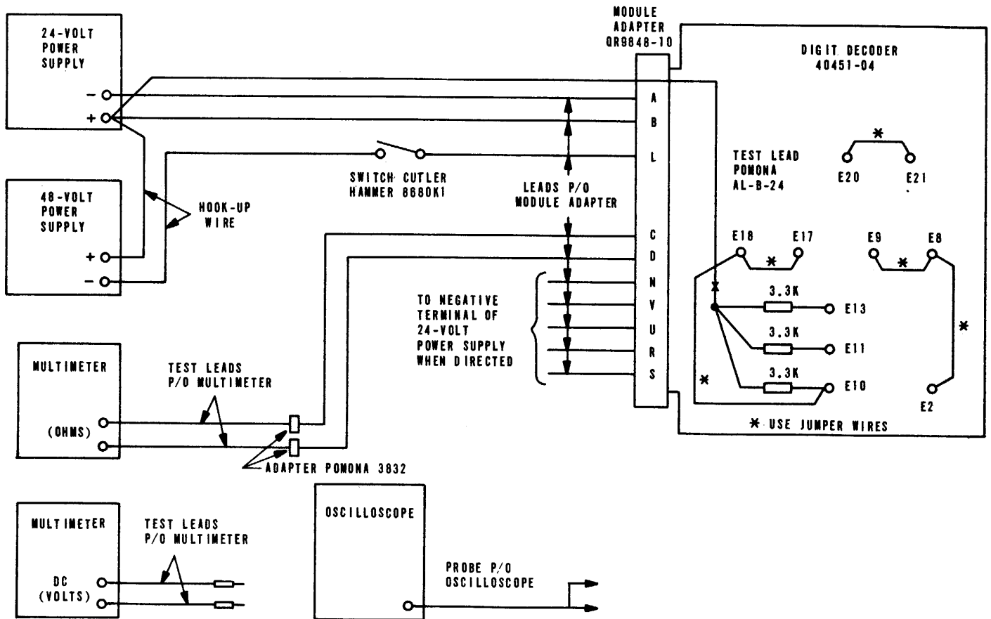
Figure 6-14. Digit Decoder 40451-04, initial test setup diagram.
