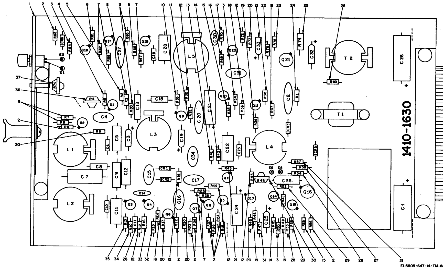
Figure 22. SF detector and oscillator 41063-02, resistor location.
