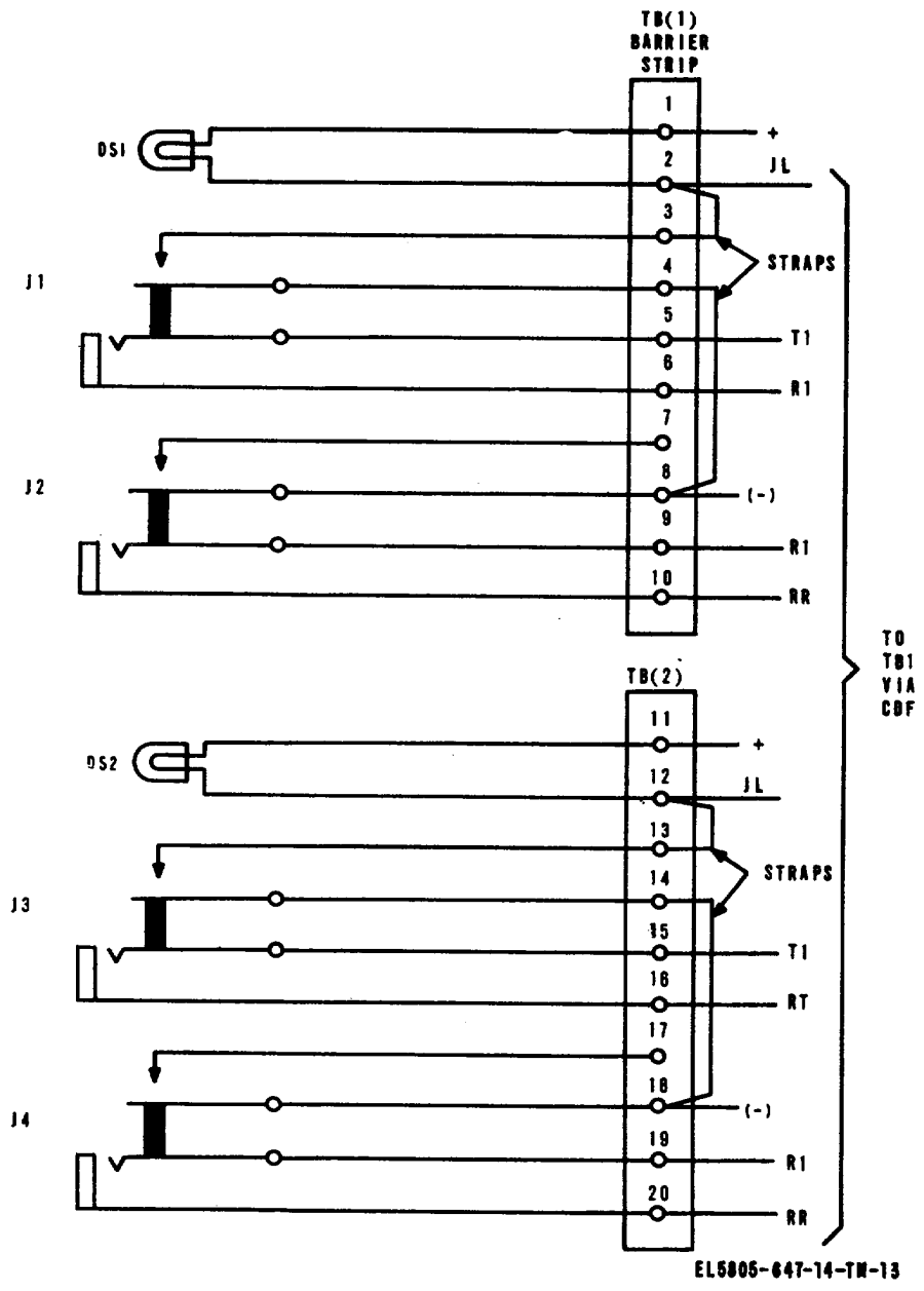
Figure 2-10. Jack and Lamp and Lamp Panel JLP-1, strapping connections.
