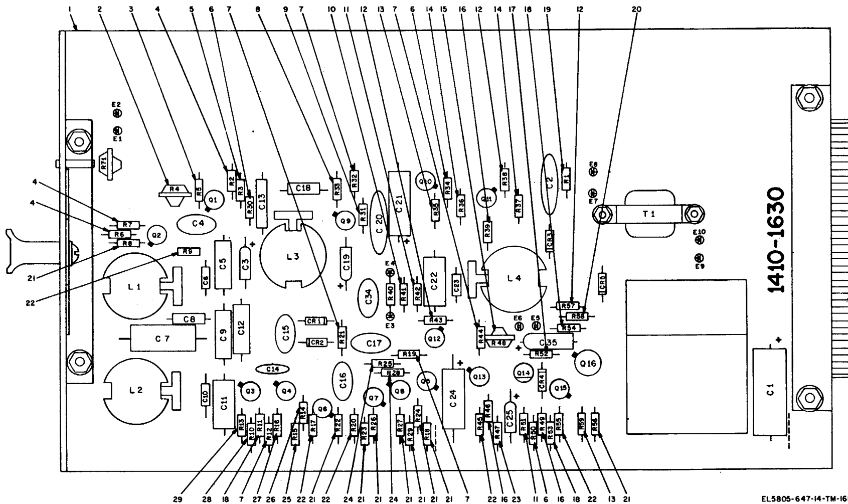
Figure 26. SF detector 41063-01, resistor location.
