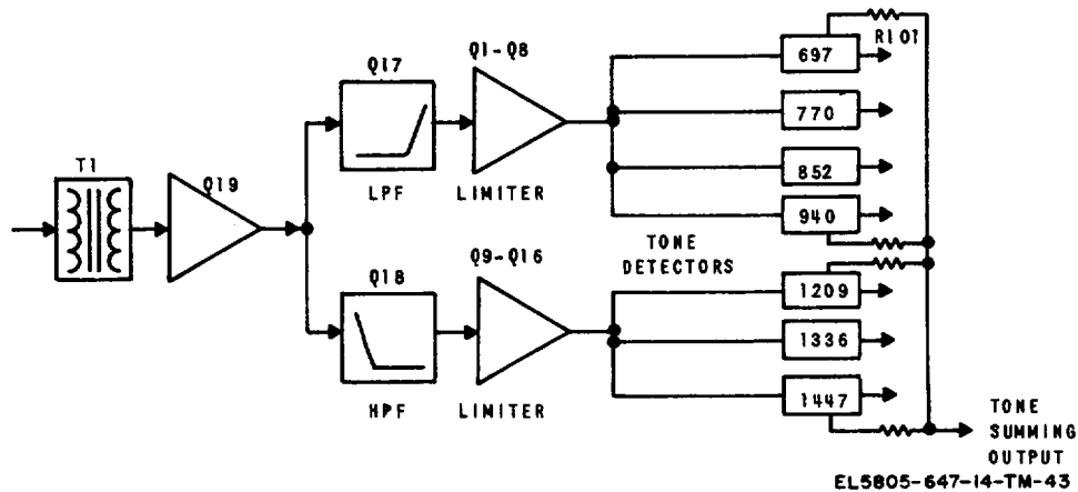
Figure 4-14. DTMF tone receiver 40452-02, simplified block diagram.
