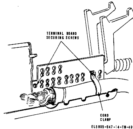
Figure 5-4. Express-Link-Local-Order Wire Unit TA-923/FSC, terminal board and line cord mountings
