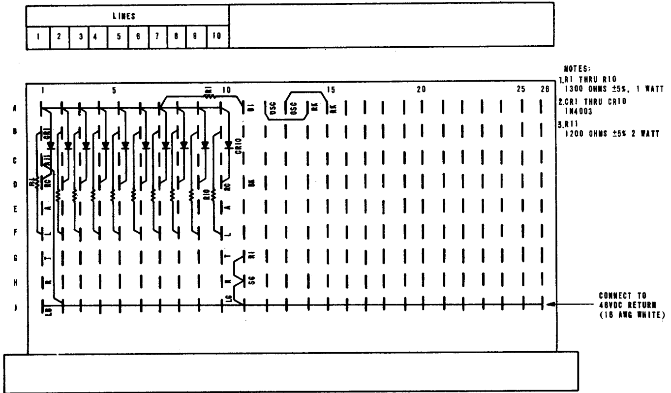
Figure 2-7. Link Orderwire Unit TA-925/FSC terminal blocks TB1/TB2 (bottom view from rear).
