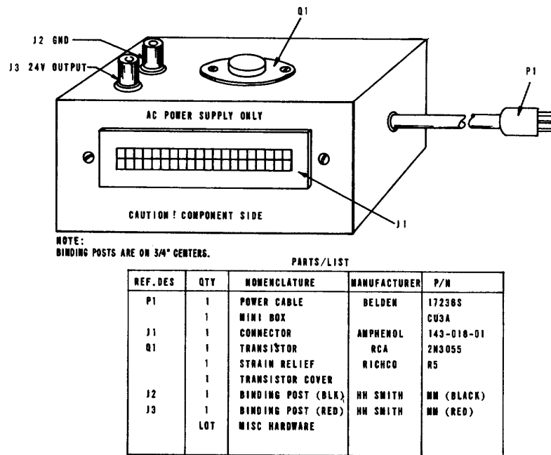
Figure 6-1. Test Adapter QR-9848-9, pictorial diagram.
