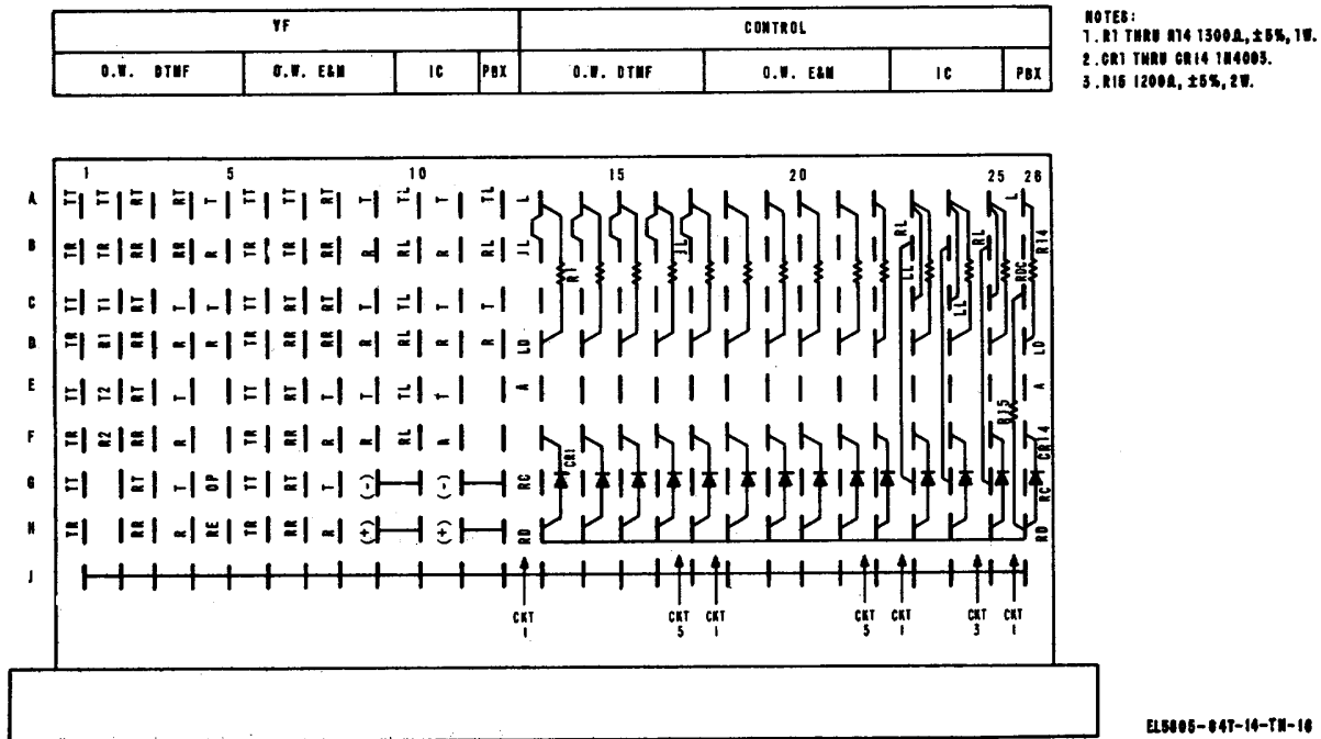
Figure 2-11. Typical terminal block TBI, EOW sites, bottom view from rear.
