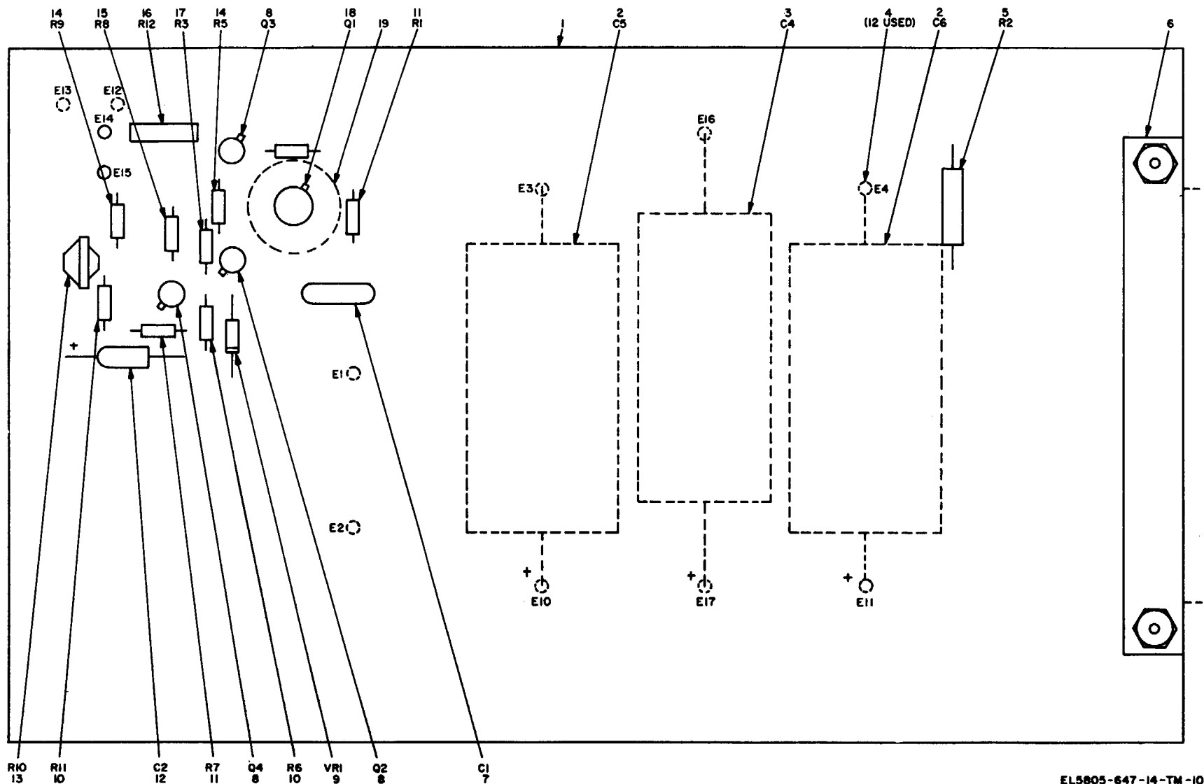
Figure 29. Printed circuit card for power supply 41028-01, parts location.
