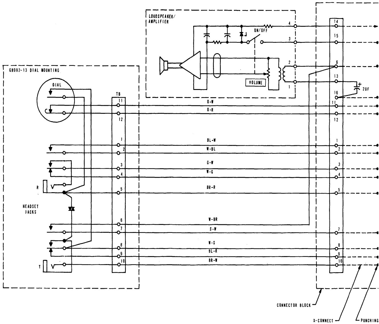
Figure FO-1(1). Express-Link-Local Orderwire Unit TA-928/FSC, wiring diagram (sheet 1 of 4).
