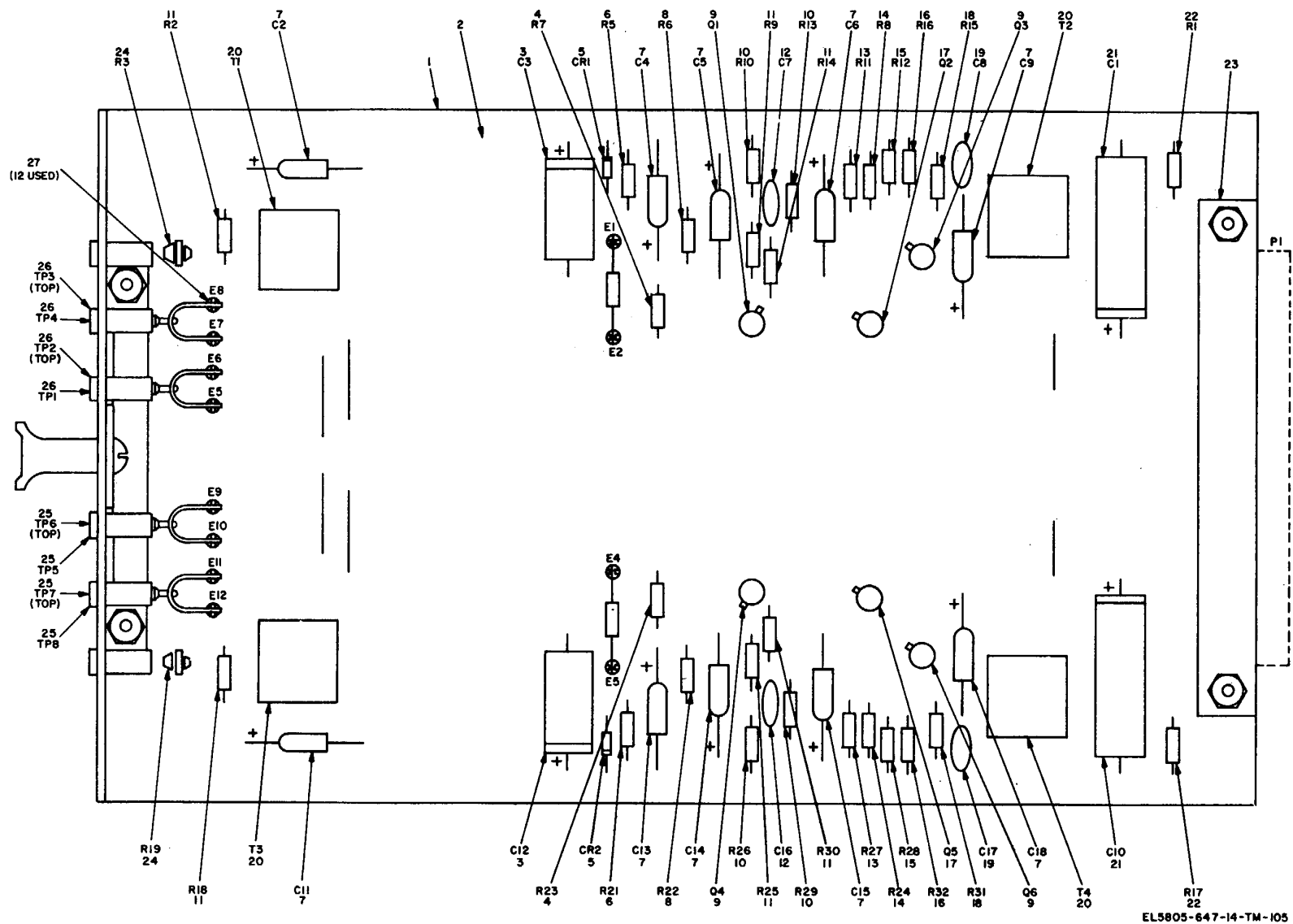
Figure 31. Dual amplifier 40472-03, parts location.
