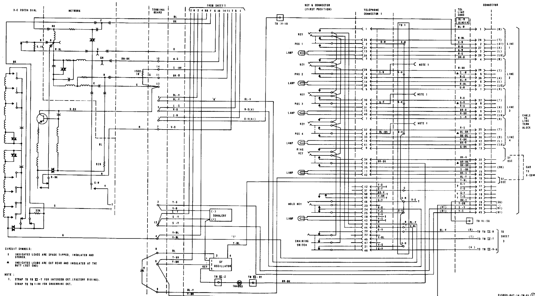
Figure FO-5(2). Remote Link Orderwire Unit TA-924/FSC, wiring diagram (sheet 2 of 3)
