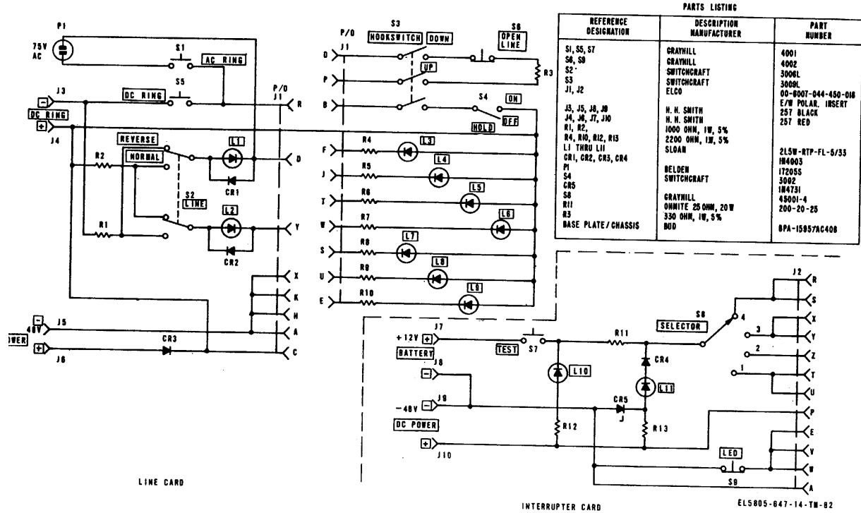
Figure 6-6. Test Adapter QR-9885, schematic diagram.
