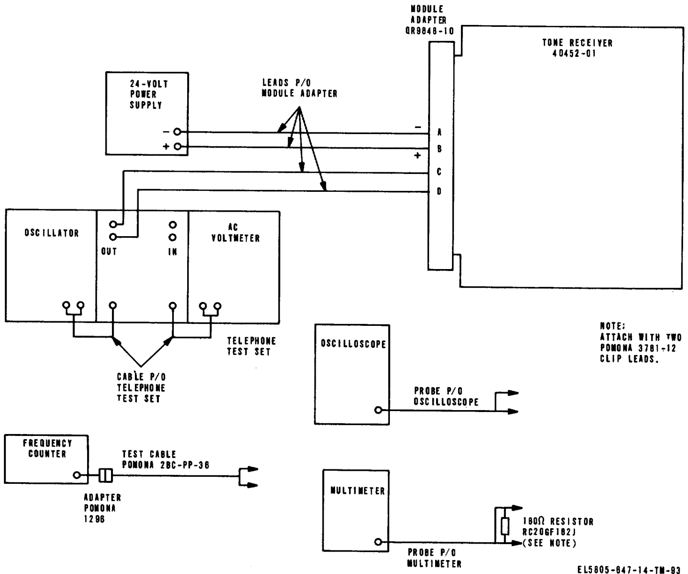
Figure 6-13. Tone Receiver 40452-01, initial test setup diagram.
