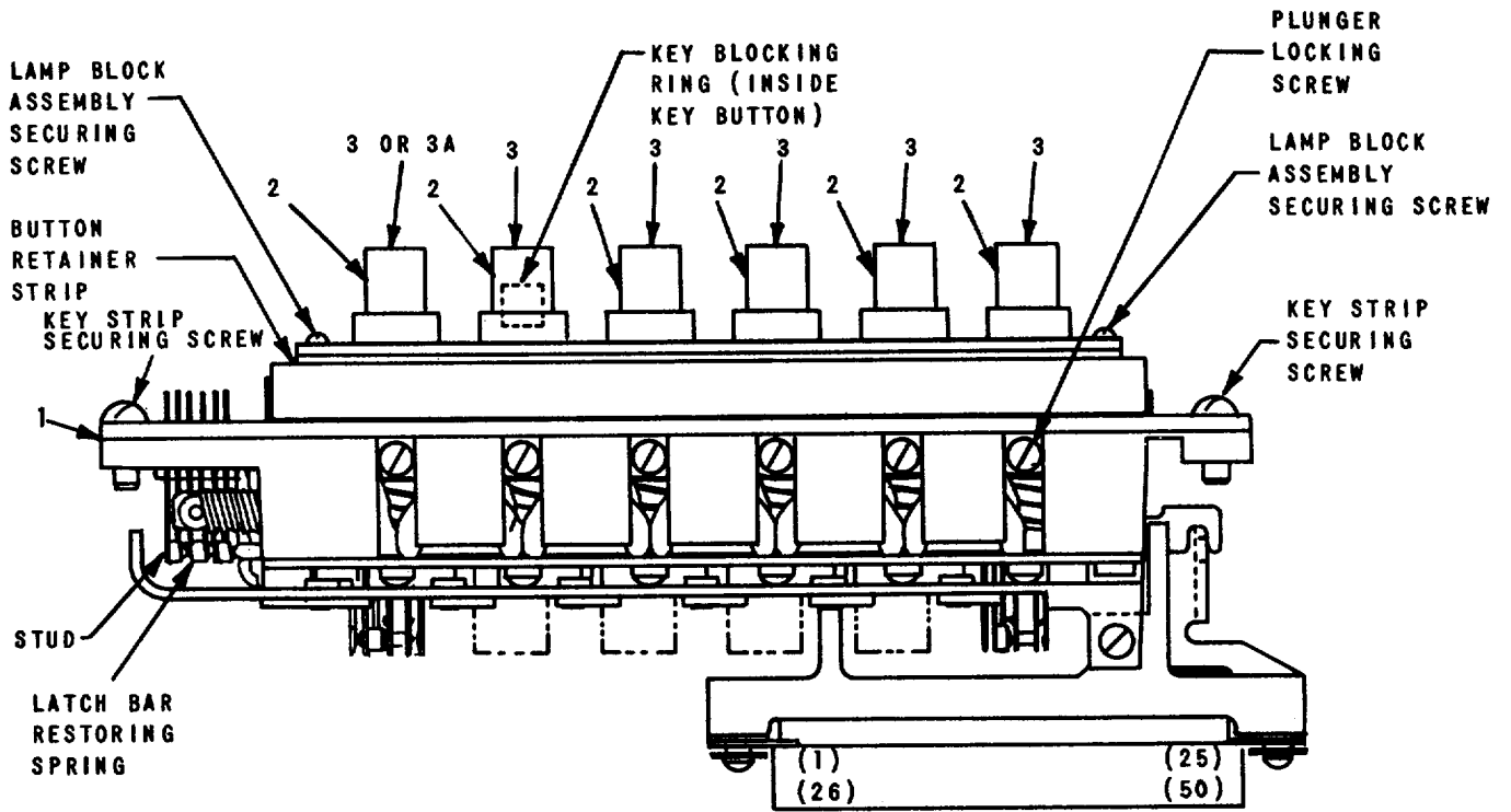
Figure 3. Typical key strip detail, parts location
