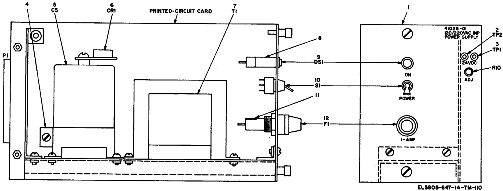
Figure 37. Power supply 41029-01, parts location.
