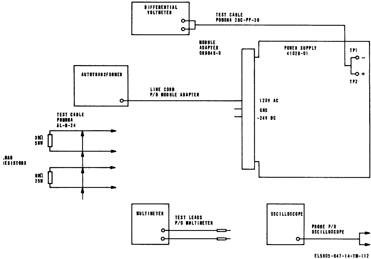
Figure 6-20. Power supply 41029-01, initial test setup diagram.
