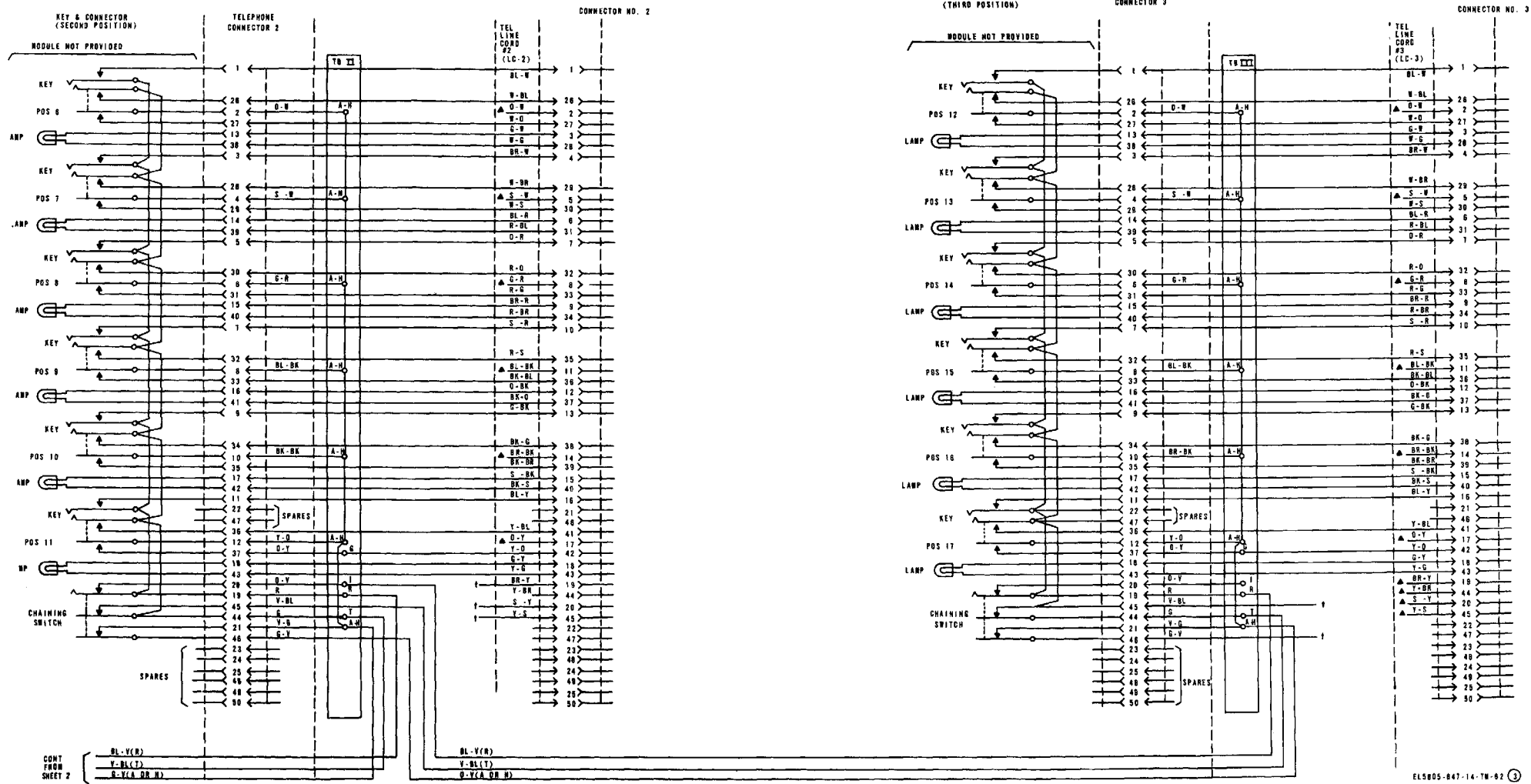
Figure FO-4(3). Remote Link Orderwire Unit TA-924/FSC, wiring diagram (sheet 3 of 3)
