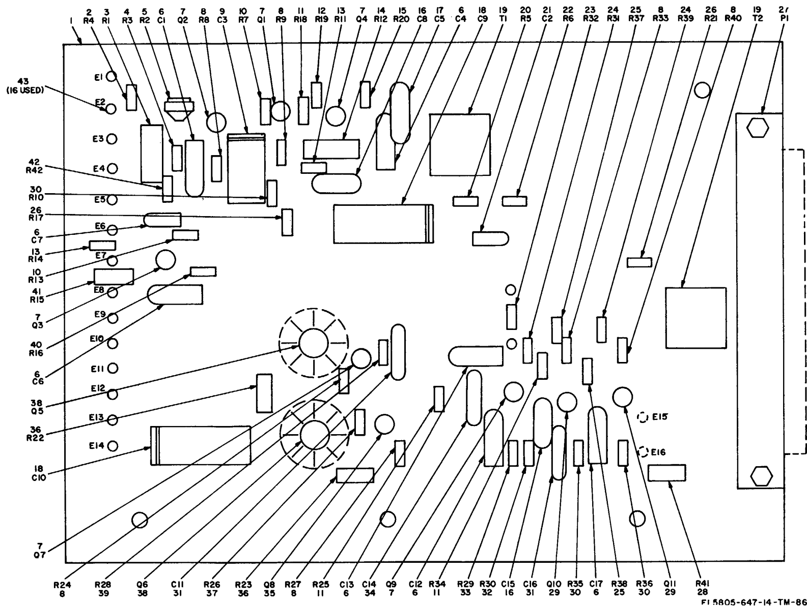
Figure 40. Printed circuit card for speaker amplifier assembly 41030-01, parts location.
