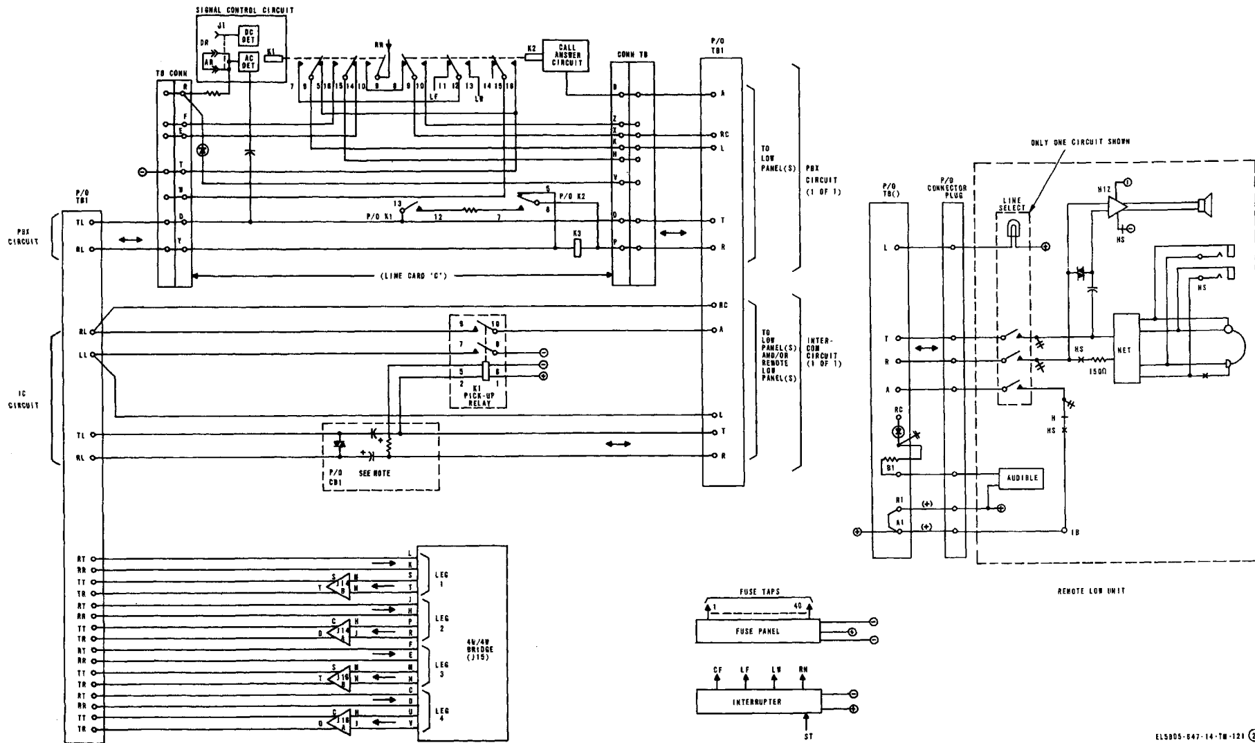
Figure FO-9(2). Orderwire/intercom (LOW sites), functional diagram (sheet 2 of 2).
