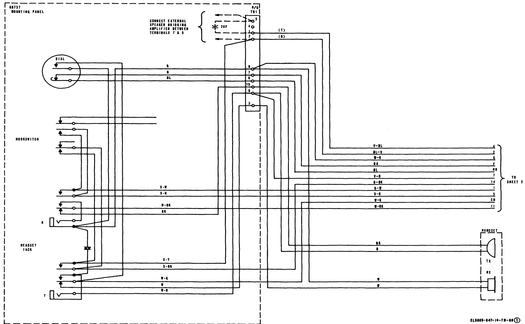
Figure FO-3(1). Express-Link-Local Orderwire Unit TA-923/FSC, wiring diagram (sheet 1 of 4).
