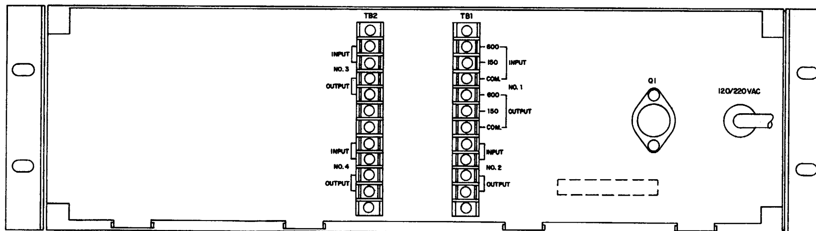
Figure 36. Local orderwire unit 411010-97, connection terminal (rear ).
