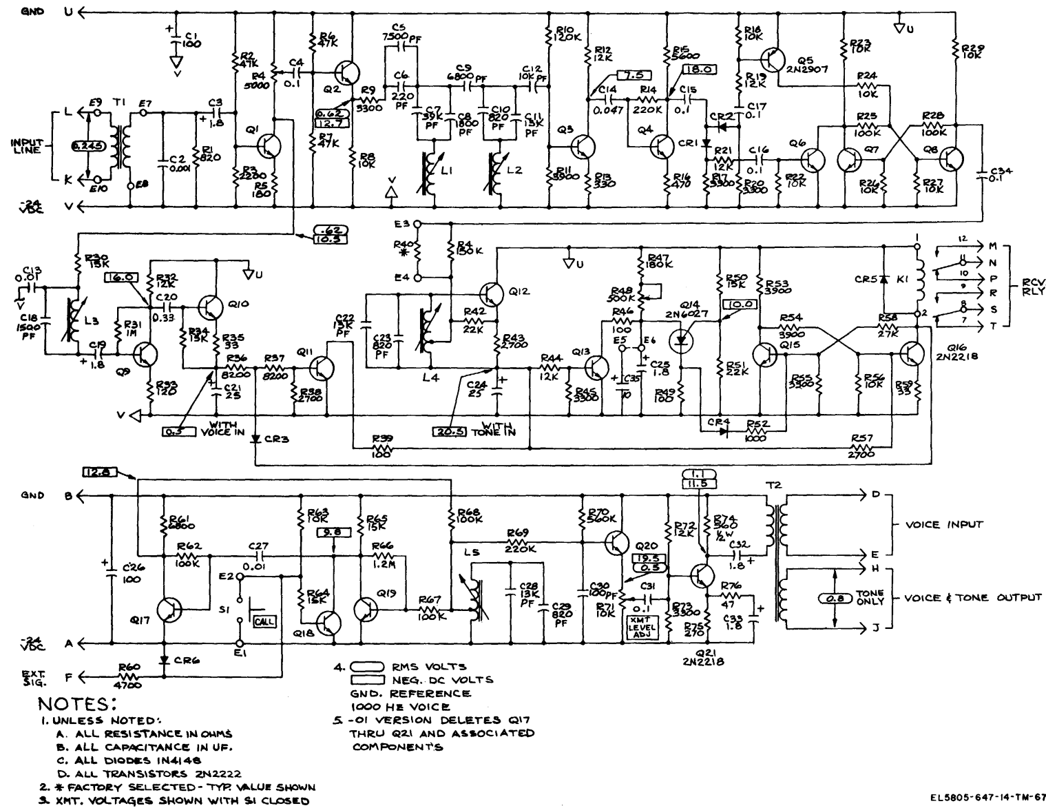
Figure FO-11. S.F. detector and oscillator 41063-02, schematic diagram.
