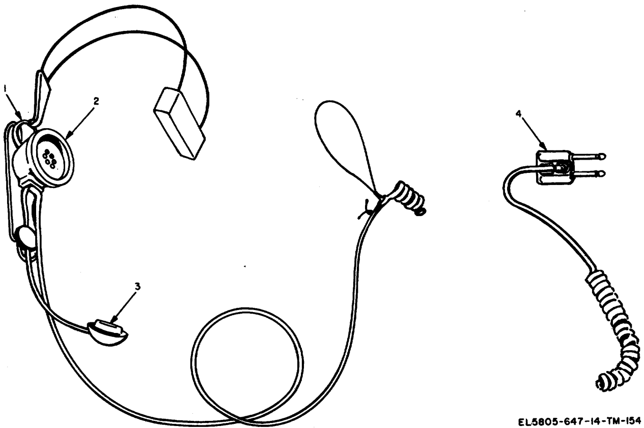
Figure 5. Headset, parts location
