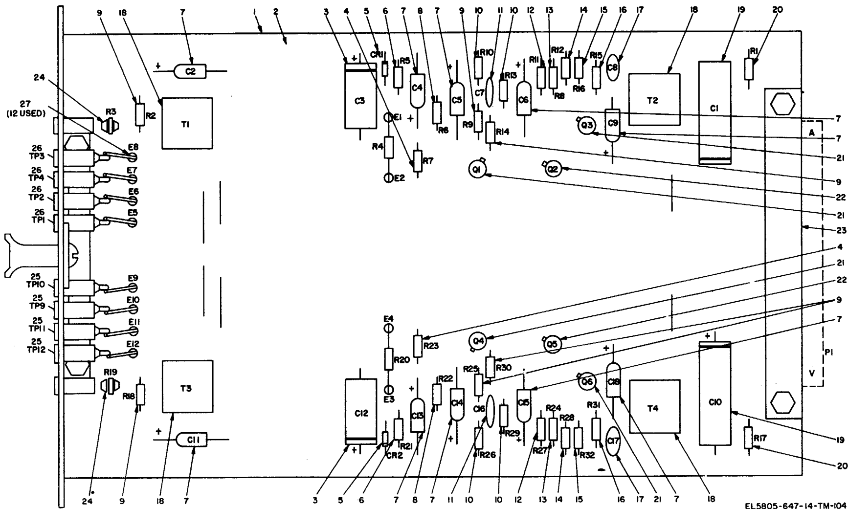
Figure 33. Dual amplifier 40172-03, parts location.
