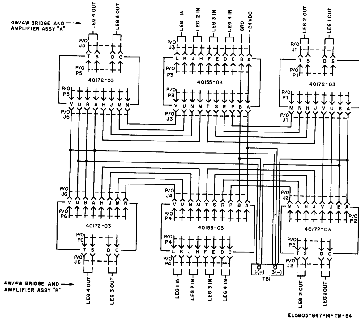
Figure FO-7. 4-Way/4-wire bridge and amplifier assembly 40155-03, intrawiring diagram.
