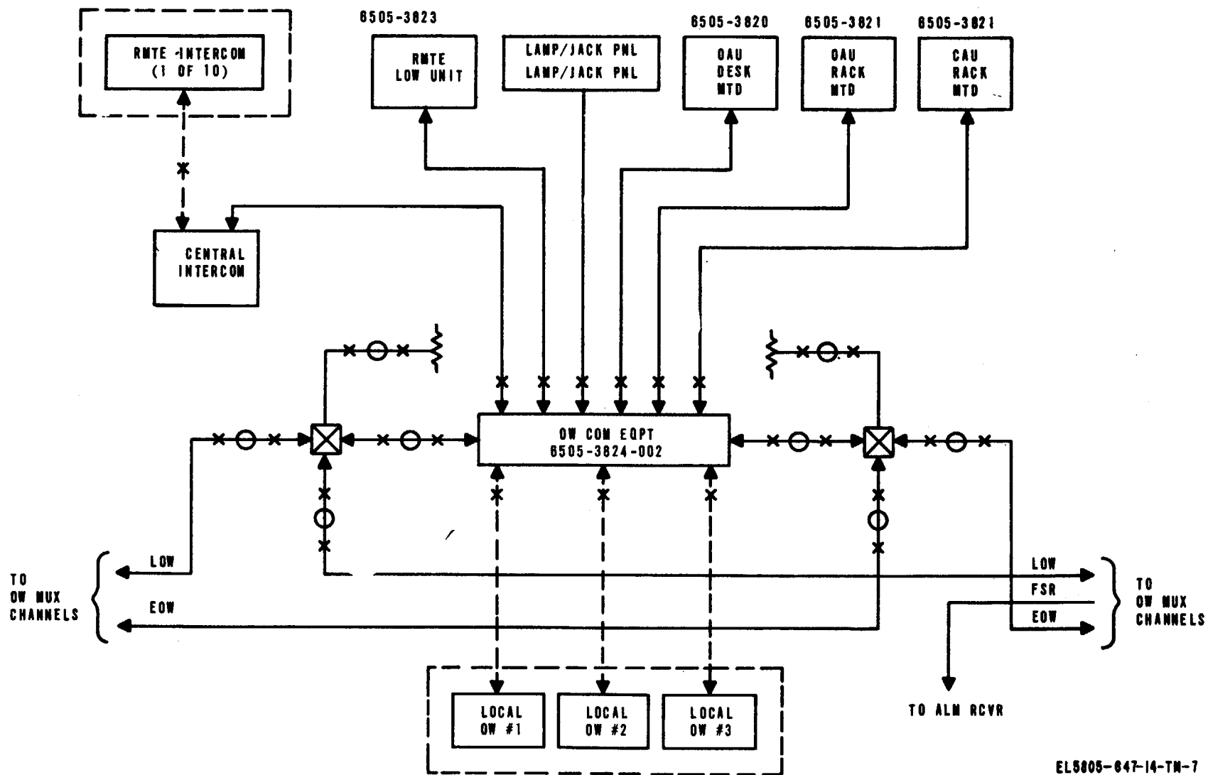
Figure 1-8. Typical, orderwire/intercom EOW station equipment arrangement, block diagram.
