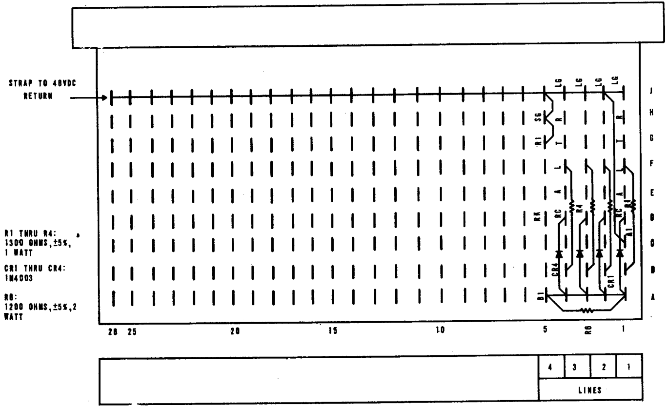
Figure 2-8. Remote Link Orderwire Unit TA-924/FSC, terminal block TB2 (bottom view from rear).
