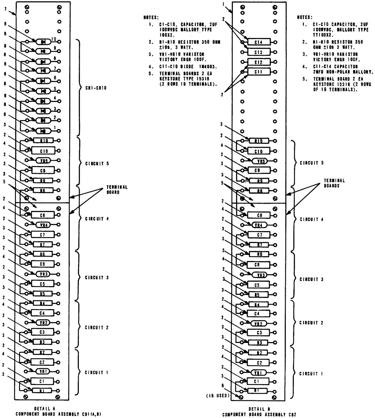
Figure 41. Typical equipment cabinet, subassembly parts location.
