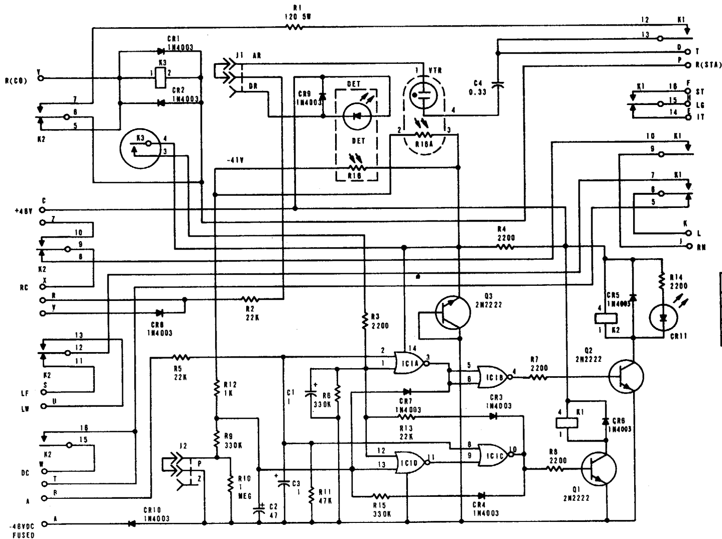
Figure 4-6. Line card LCC9740, schematic diagram.
