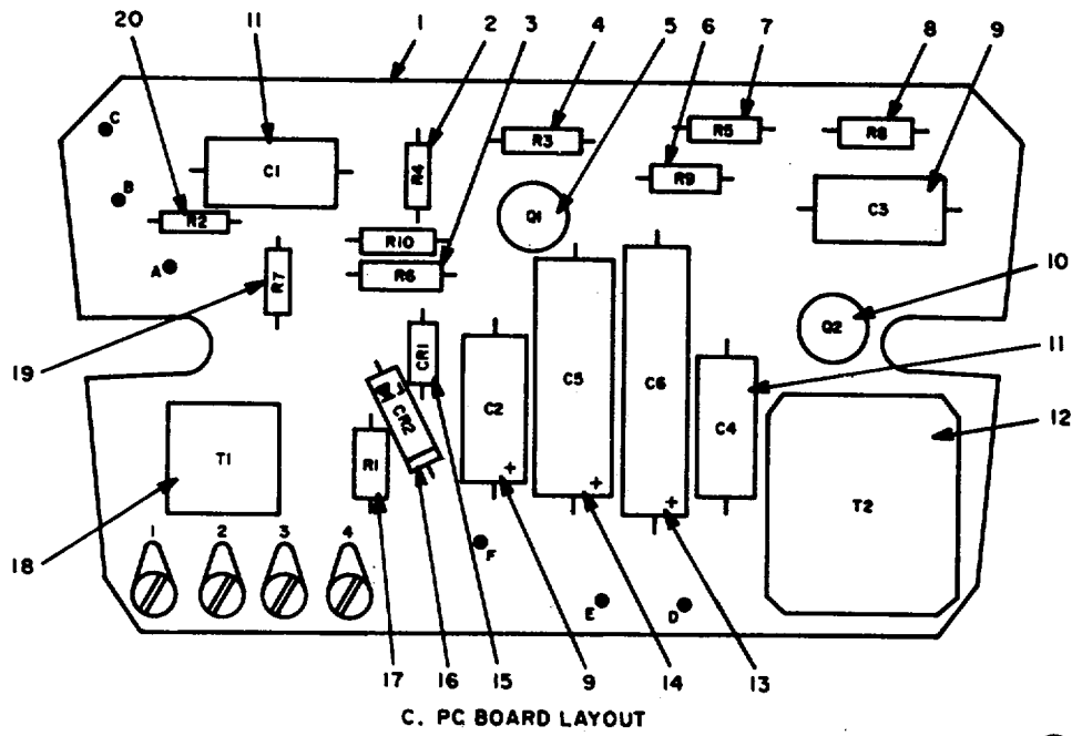
Figure 13. Speaker amplifier unit -3828, parts location.
