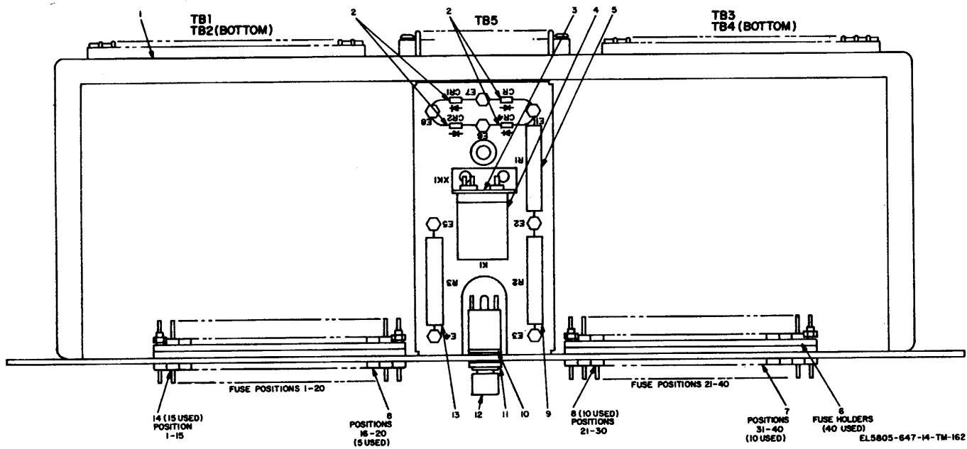
Figure 14. Fuse panel SB-751/FSC, parts location.
