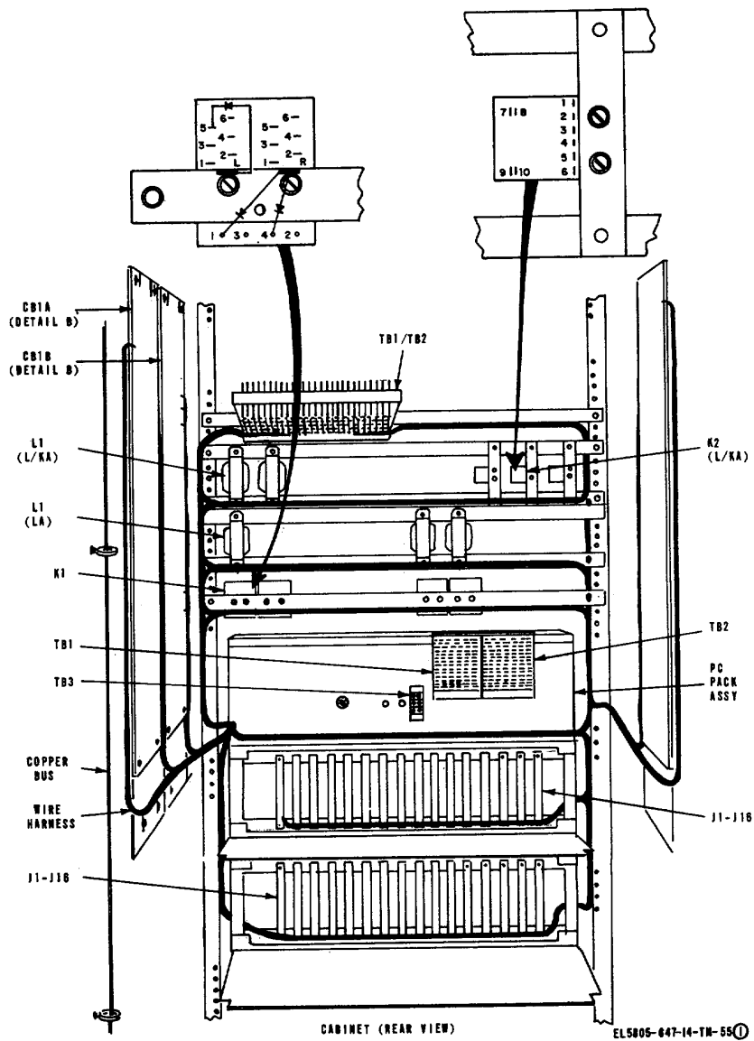
Figure 5-9. Typical equipment cabinet, subassembly parts location.
