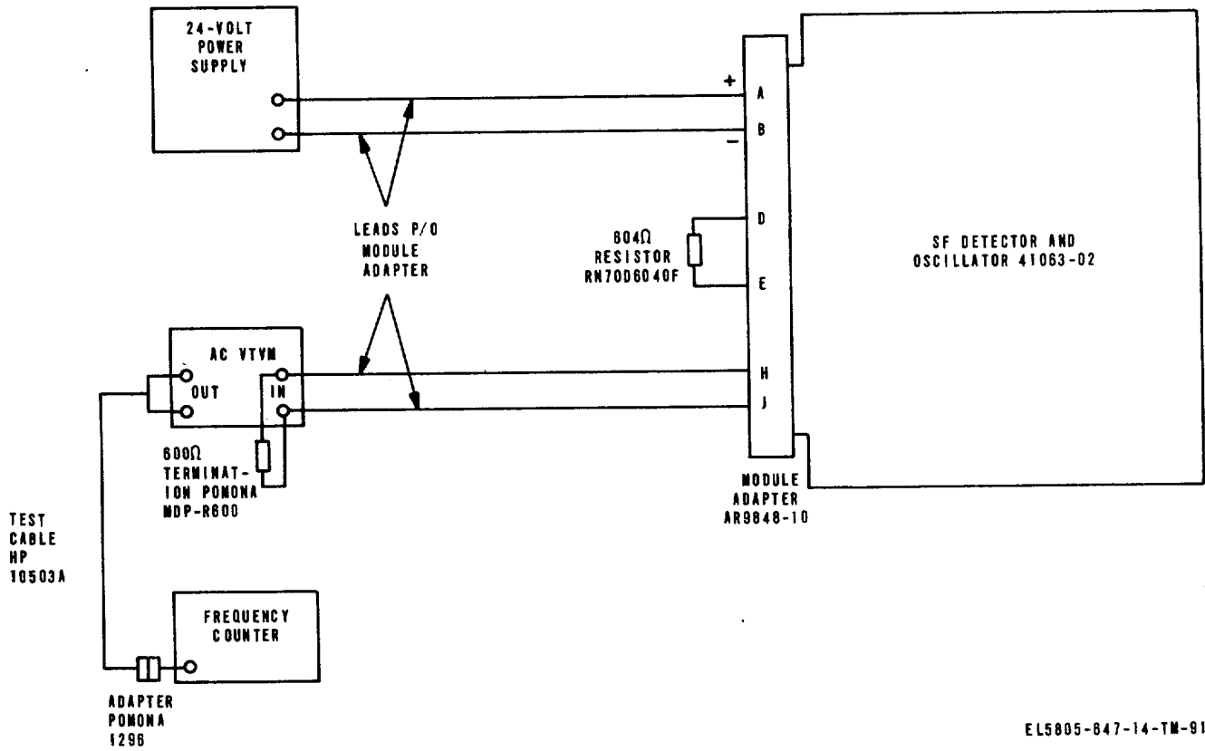
Figure 6-12. S. F. oscillator alignment, initial test setup diagram.
