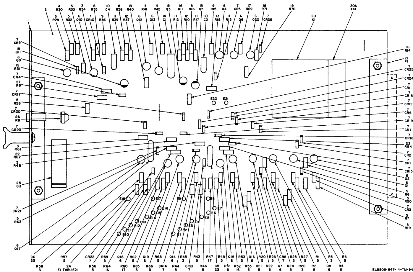
Figure 21. Digit decoder 40451-04, parts location.
