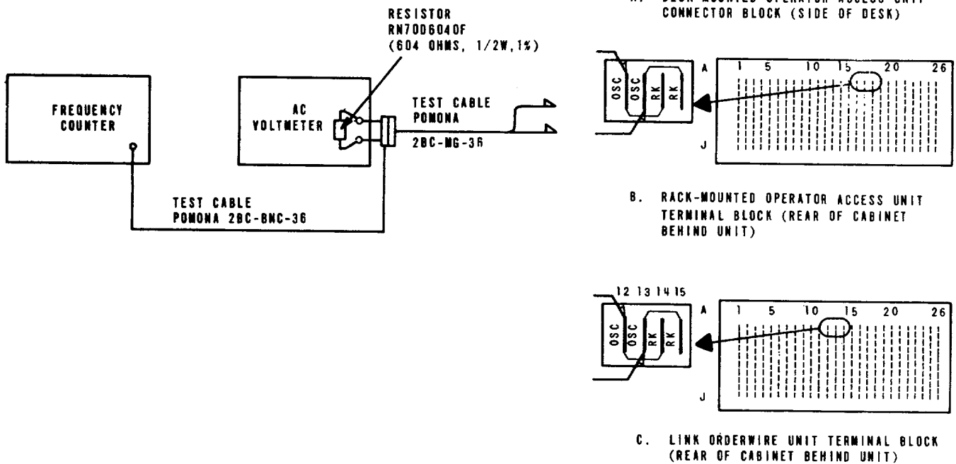
Figure 2-17. SF oscillator 49009-01, test setup diagram.
