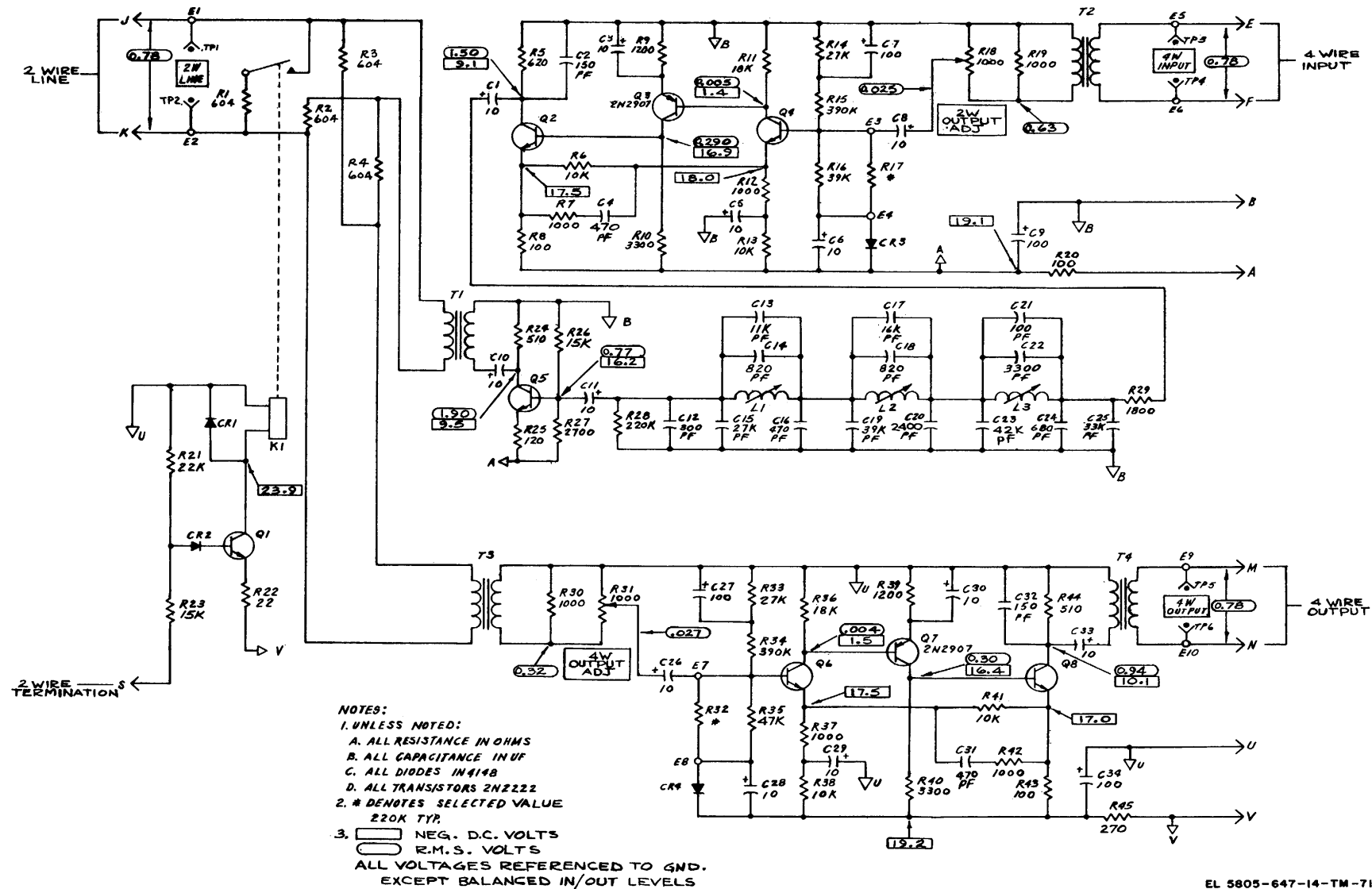
Figure FO-15. 4W/2W hybrid 4908-01, schematic diagram.
