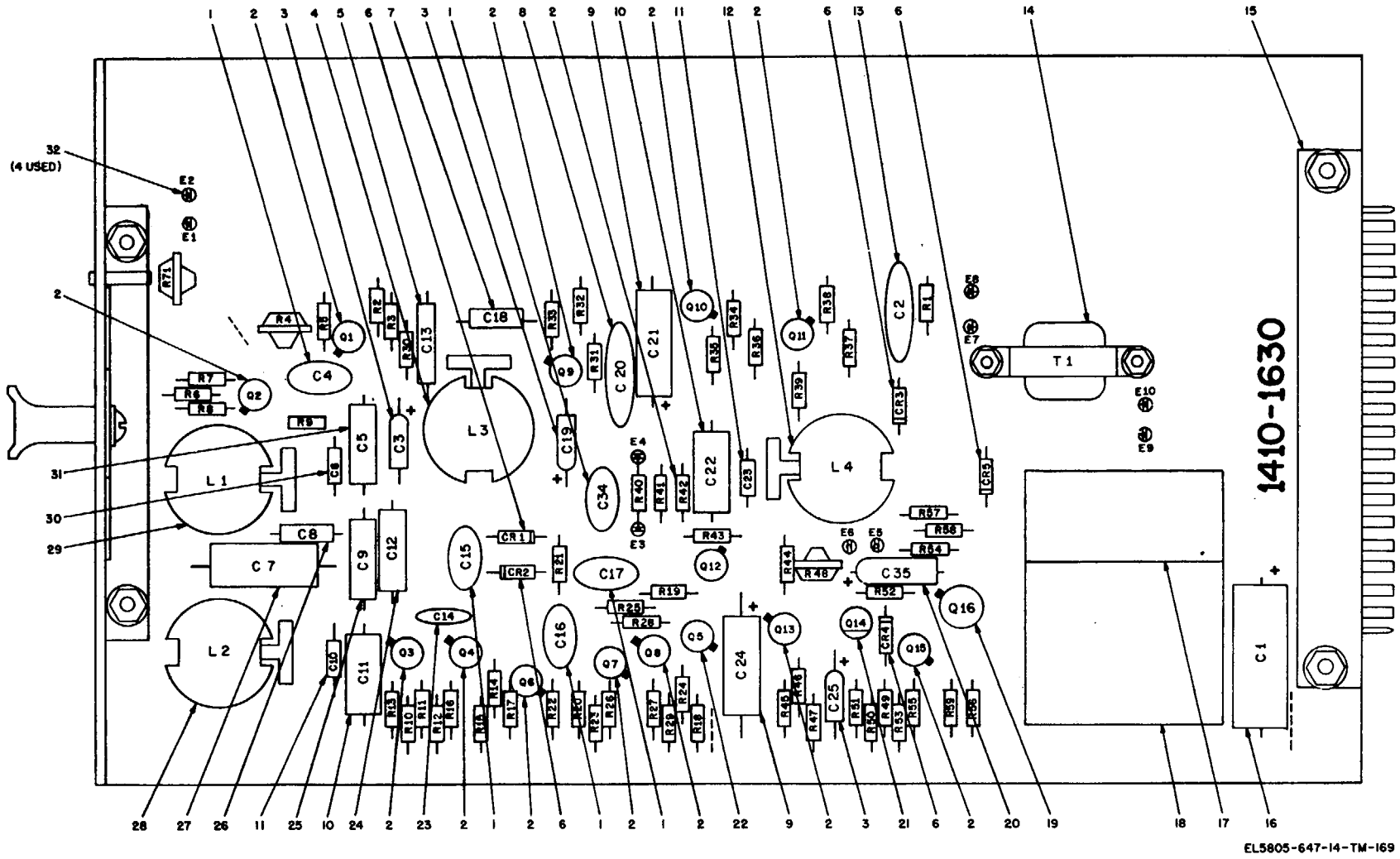
Figure 27. SF detector 41063-01, parts location.
