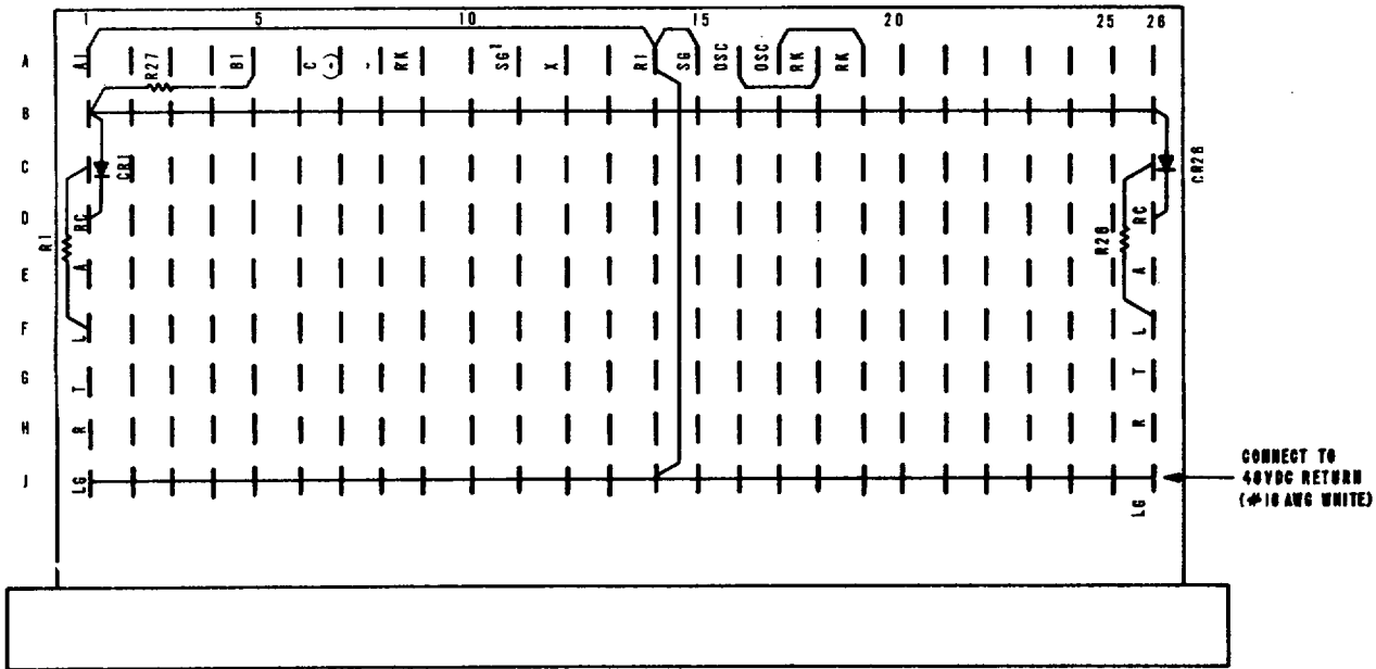
Figure 2-6. Express-Link-Local Order Wire Unit TA-923/FSC, terminal block, TB1 (bottom view from rear).
