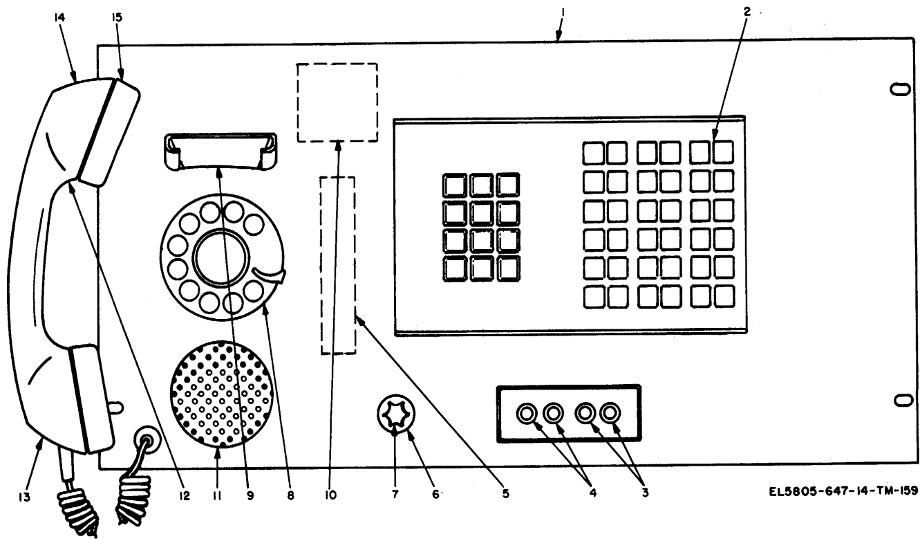
Figure 10. Call director panel assembly and handset, parts location.
