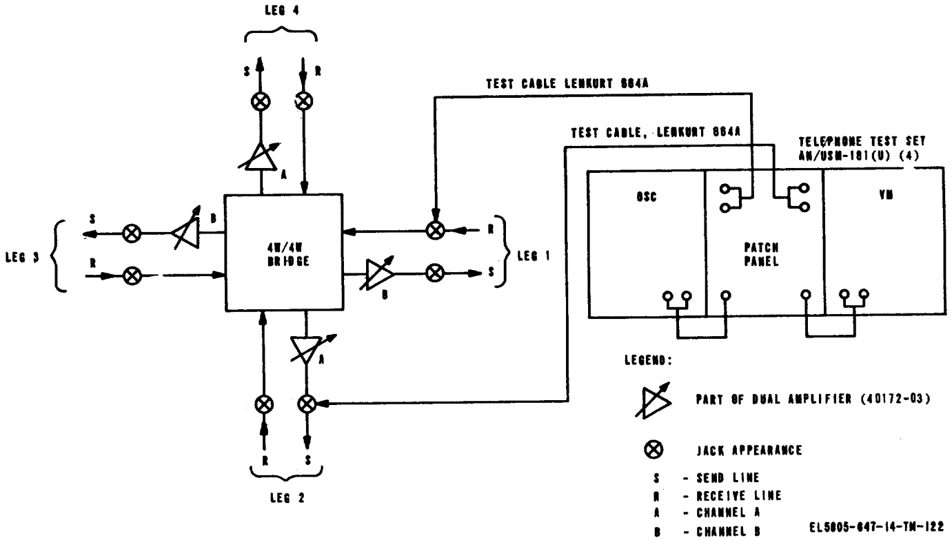
Figure 2-14. Dual amplifier, 40472-03/40172-03, test setup diagram.
