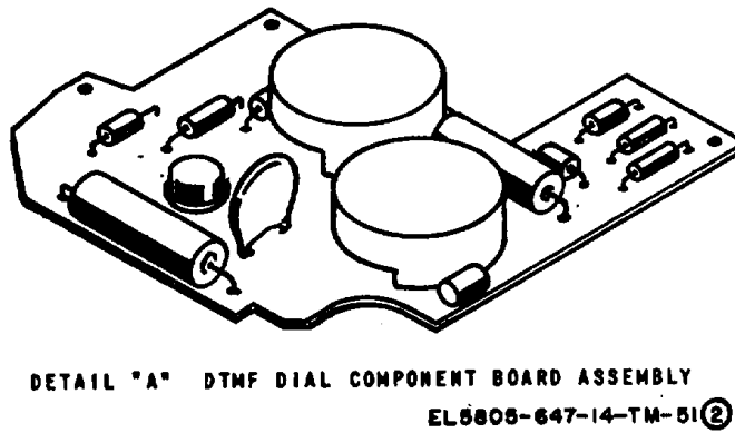
Figure 5-7 (2). 30 button key frame, component mounting, (sheet 2 of 2).
