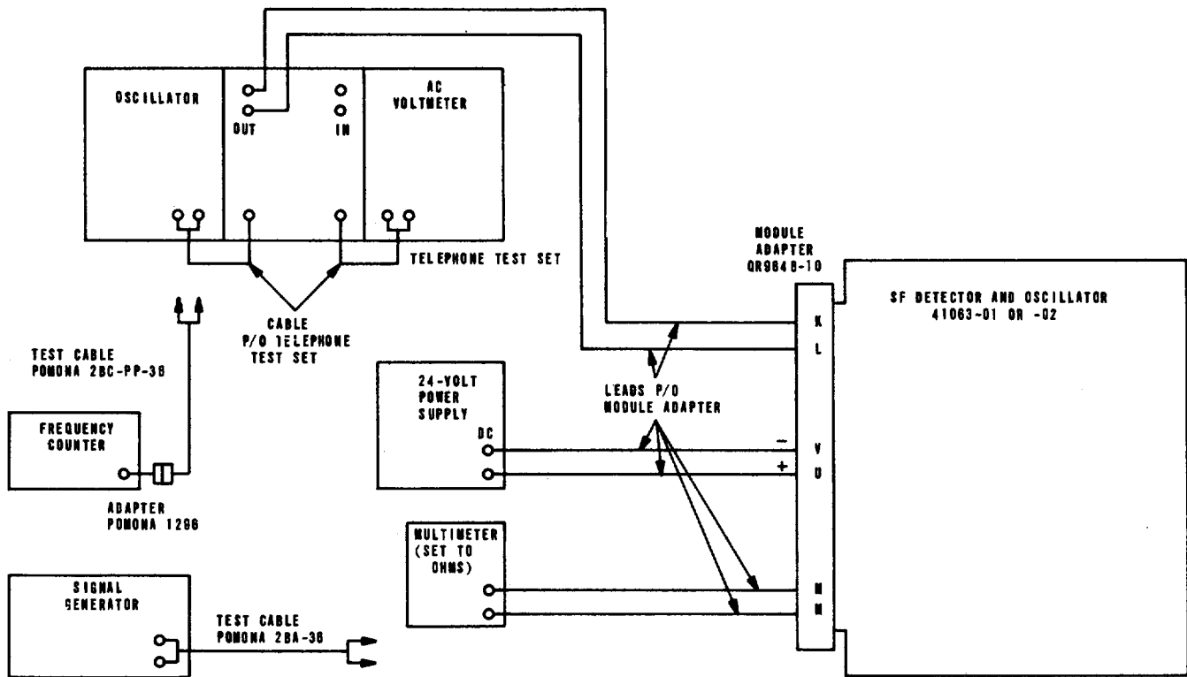
Figure 6-11. S. F. detector performance test, setup diagram.
