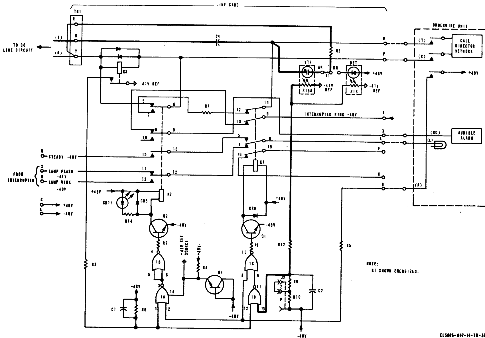
Figure 4-7. Incoming ring on PBX Line, functional diagram. 4-16
