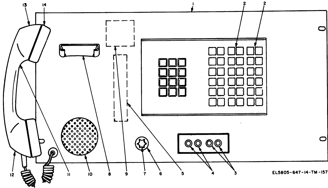
Figure 8. Call director panel assembly and handset, parts location.
