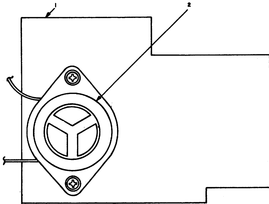
Figure 6. Buzzer assembly, parts 0141
