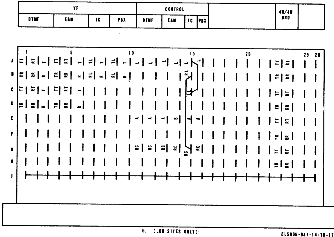
Figure 2-12. Typical terminal block TB1, LOW sites, bottom view from rear.
