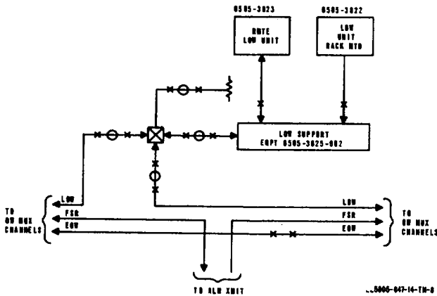
Figure 1-9. Typical, orderwire/intercom LOW station, block diagram
