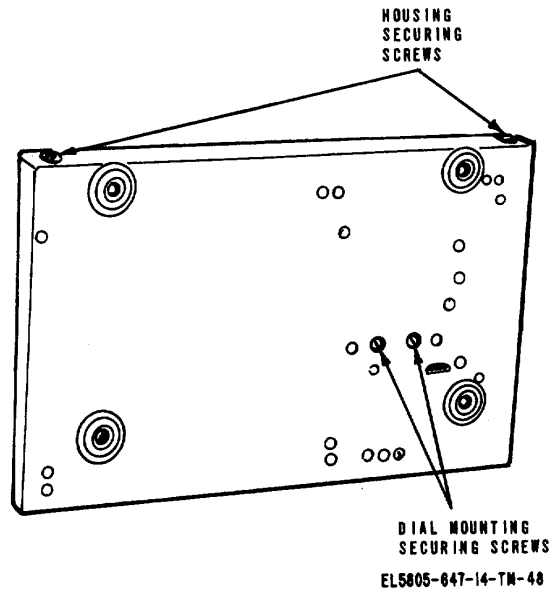
Figure 5-2. Typical telephone baseplate, mounting details
