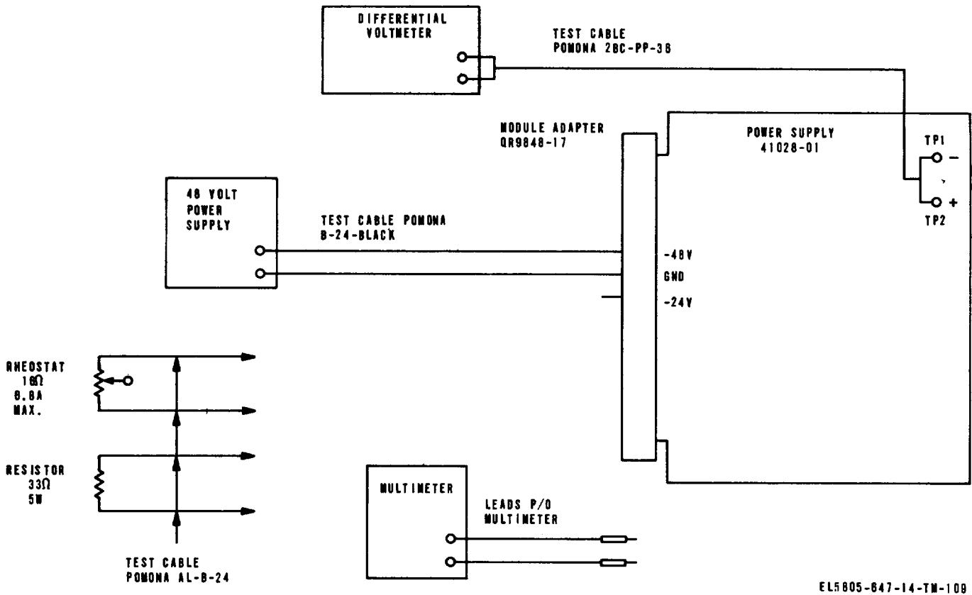
Figure 6-19. Power Supply 41028-01, initial test setup diagram.
