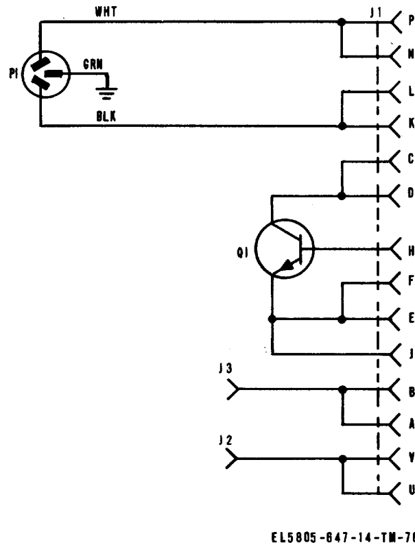
Figure 6-2. Test Adapter QR-9848-9, schematic diagram.
