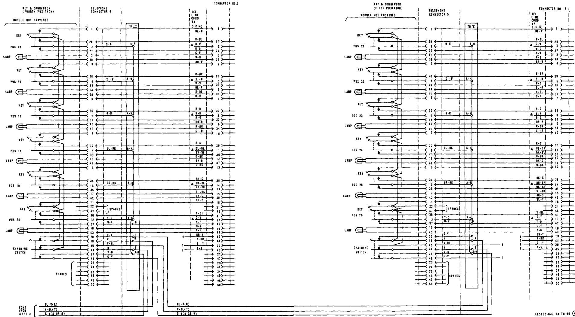
Figure FO-3(4). Express-Link-Local Orderwire Unit TA-923/FSC, wiring diagram (sheet 4 of 4).
