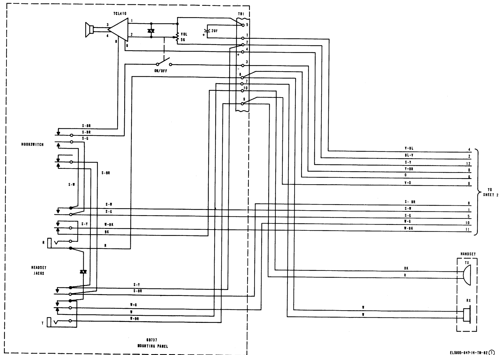
Figure FO-5(1). Remote Link Orderwire Unit TA-924/FSC, wiring diagram (sheet 1 of 3)
