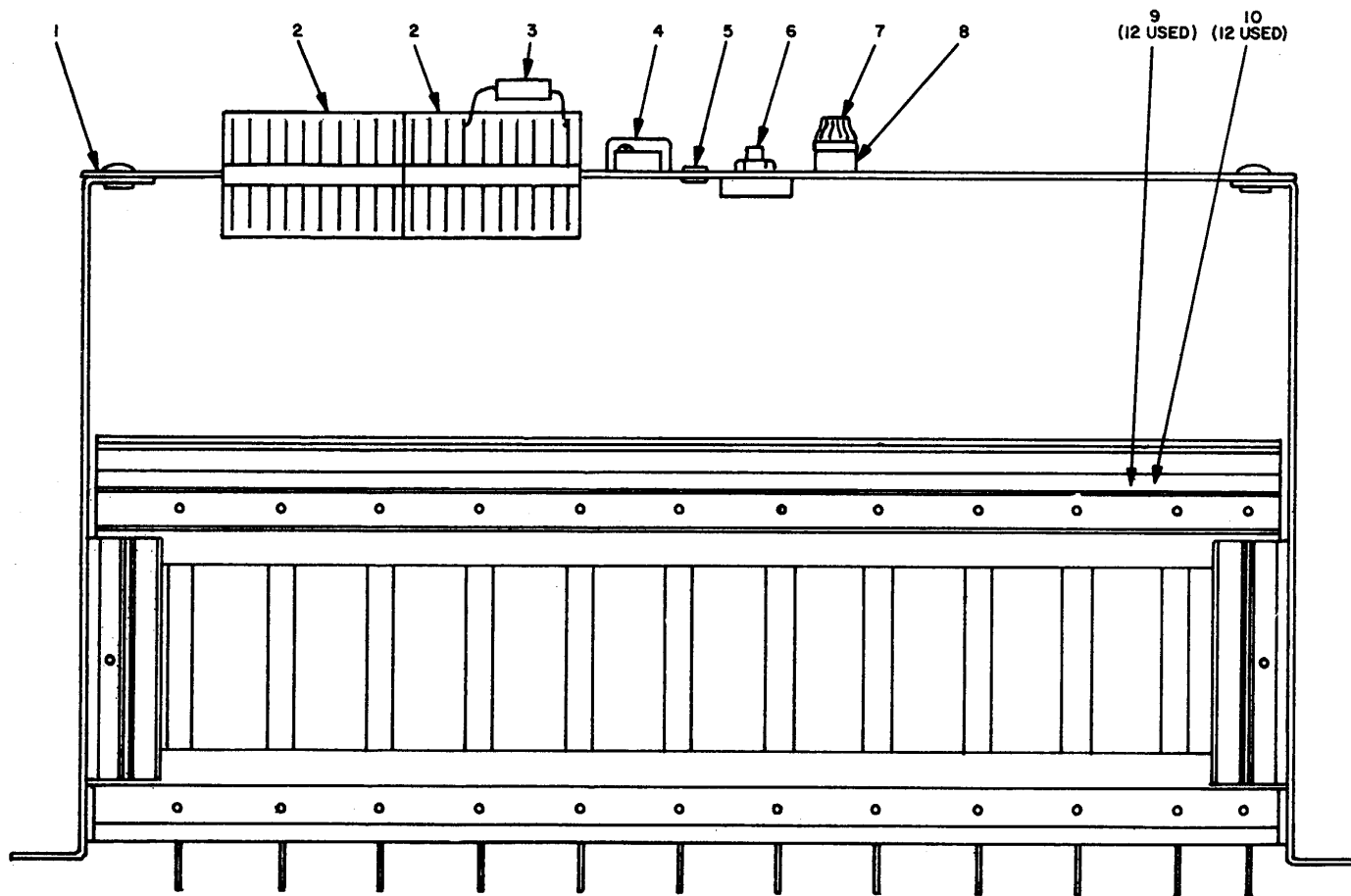
Figure 15. PC card rack assembly, parts location
