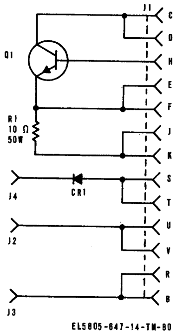
Figure 6-4. Test Adapter QR-9848-17, schematic diagram.
