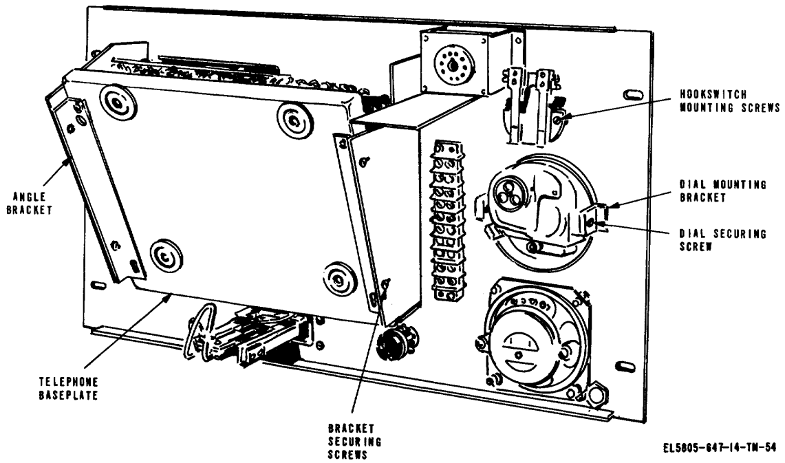
Figure 5-3. Rack mounted call director, frame and parts location (rear view).
