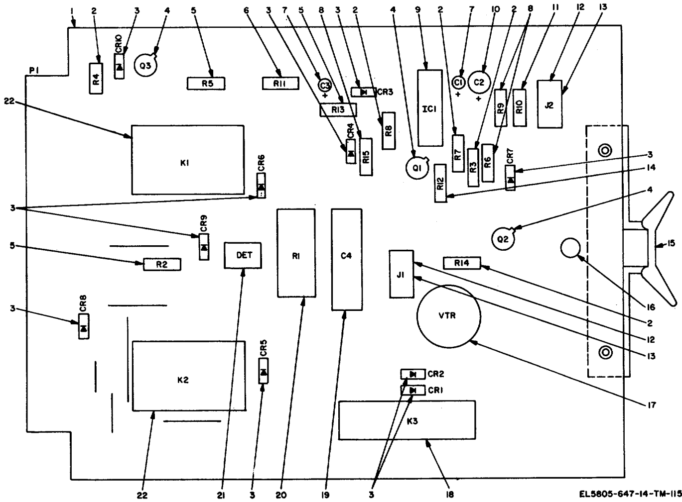
Figure 16. Line card assembly LC401-4, parts location.
