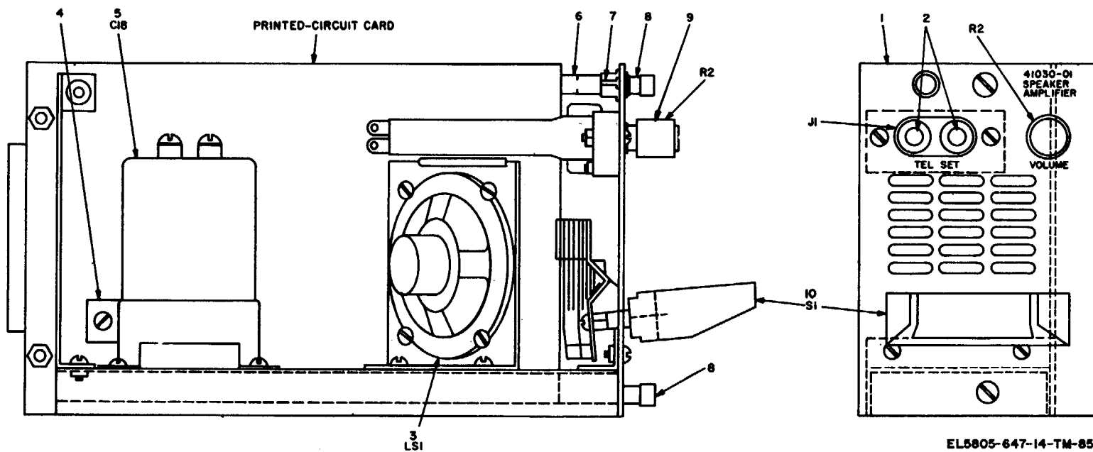
Figure 39. Speaker amplifier assembly 41030-01, parts location.
