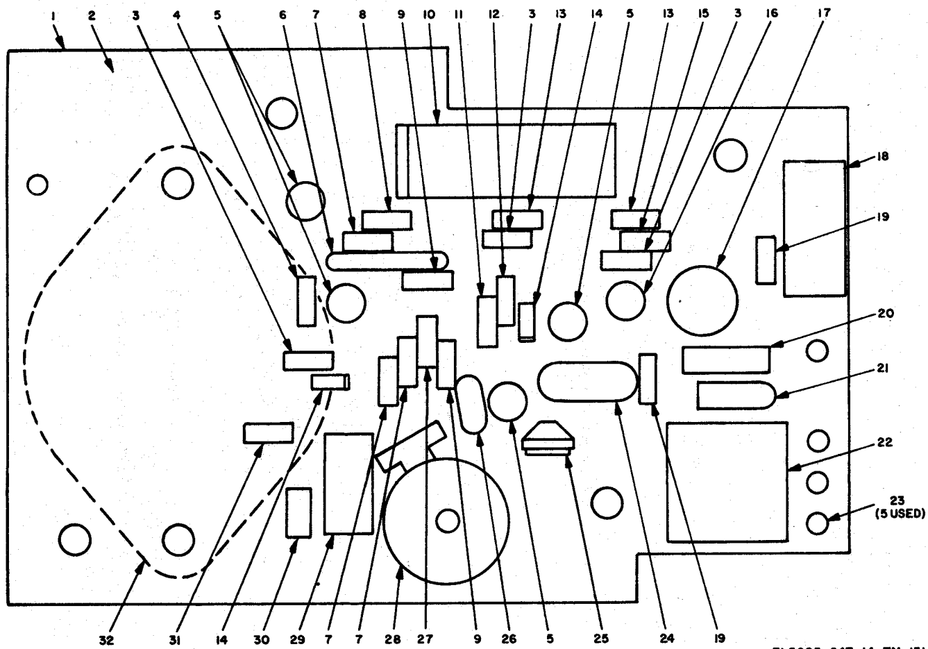
Figure 1. Oscillator assembly, parts location
